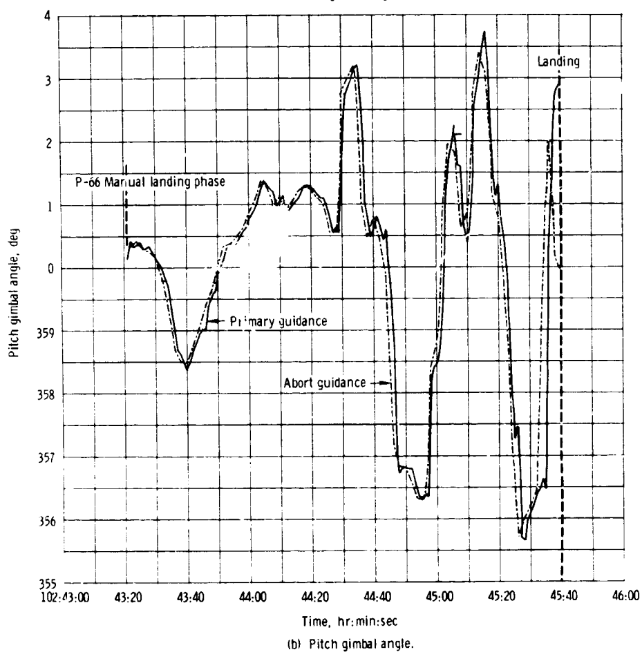
Figure 5-6. - Expanded pitch and roll attitude time histories near landing.
