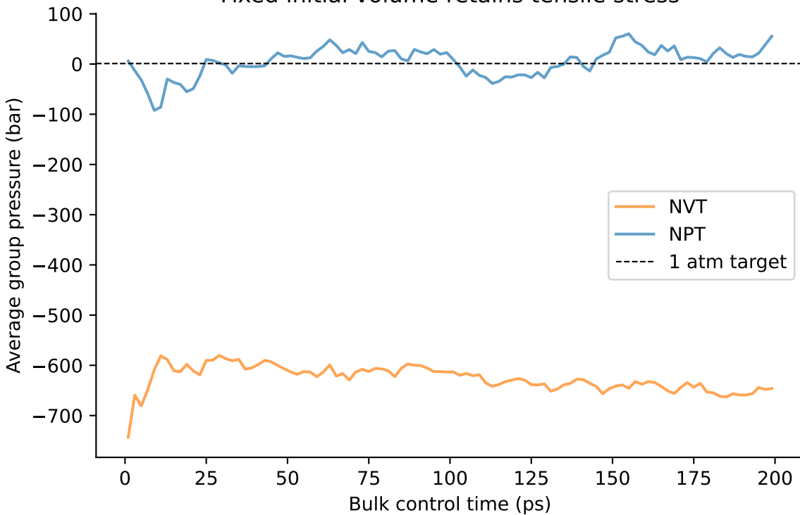
Fixed initial volume retains tensile stress
