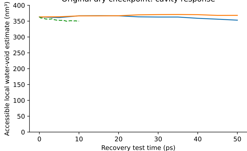
Single samples; not equilibrium averages
