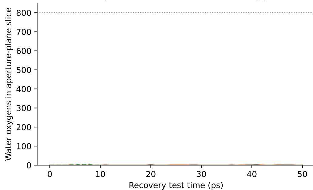
A wet aperture would contain ~800 oxygens
