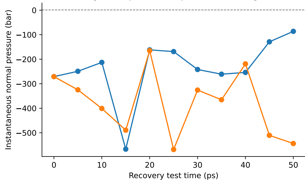
Single samples; not equilibrium averages
