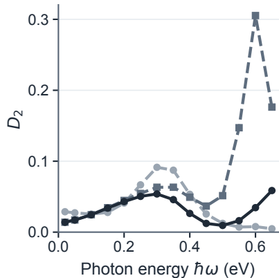
(c) CASCI anchor
