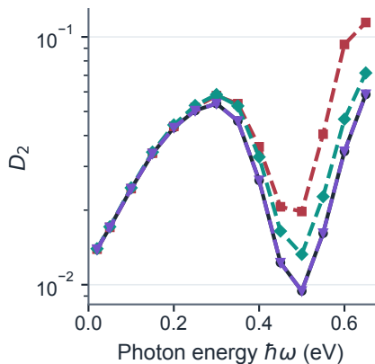
(c) CASCI anchor
