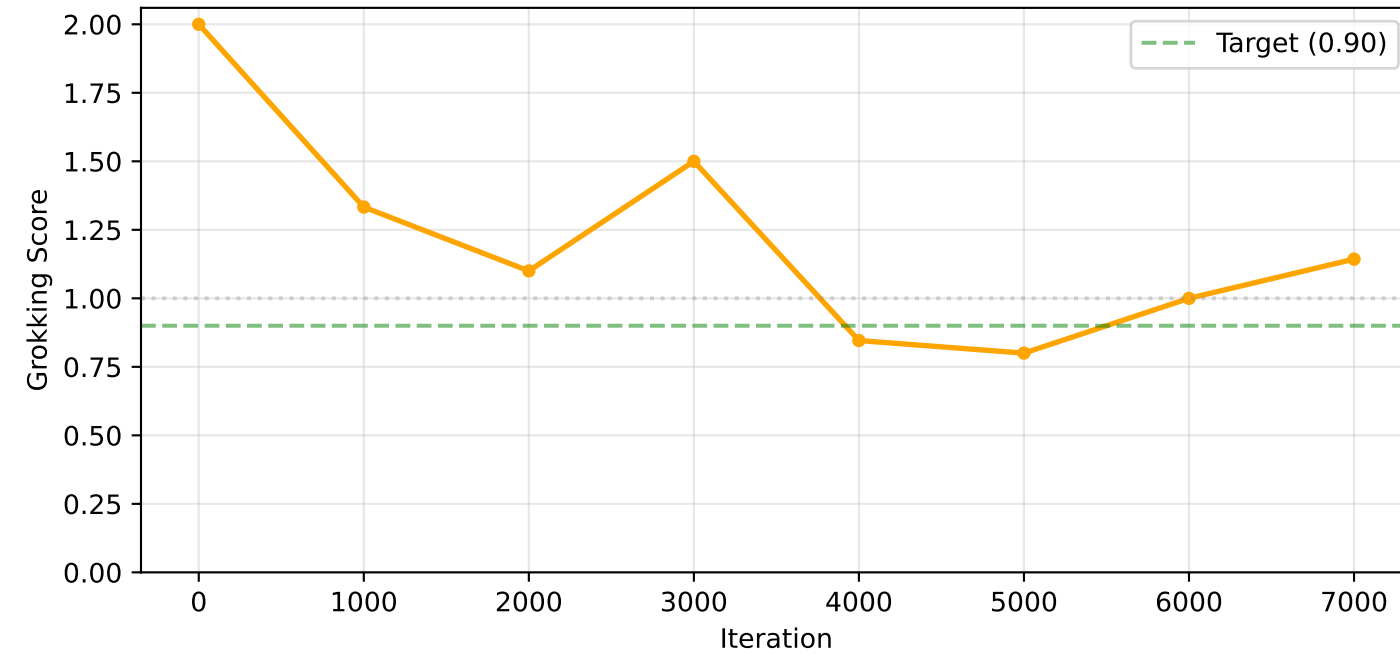
Grokking Score Progress
