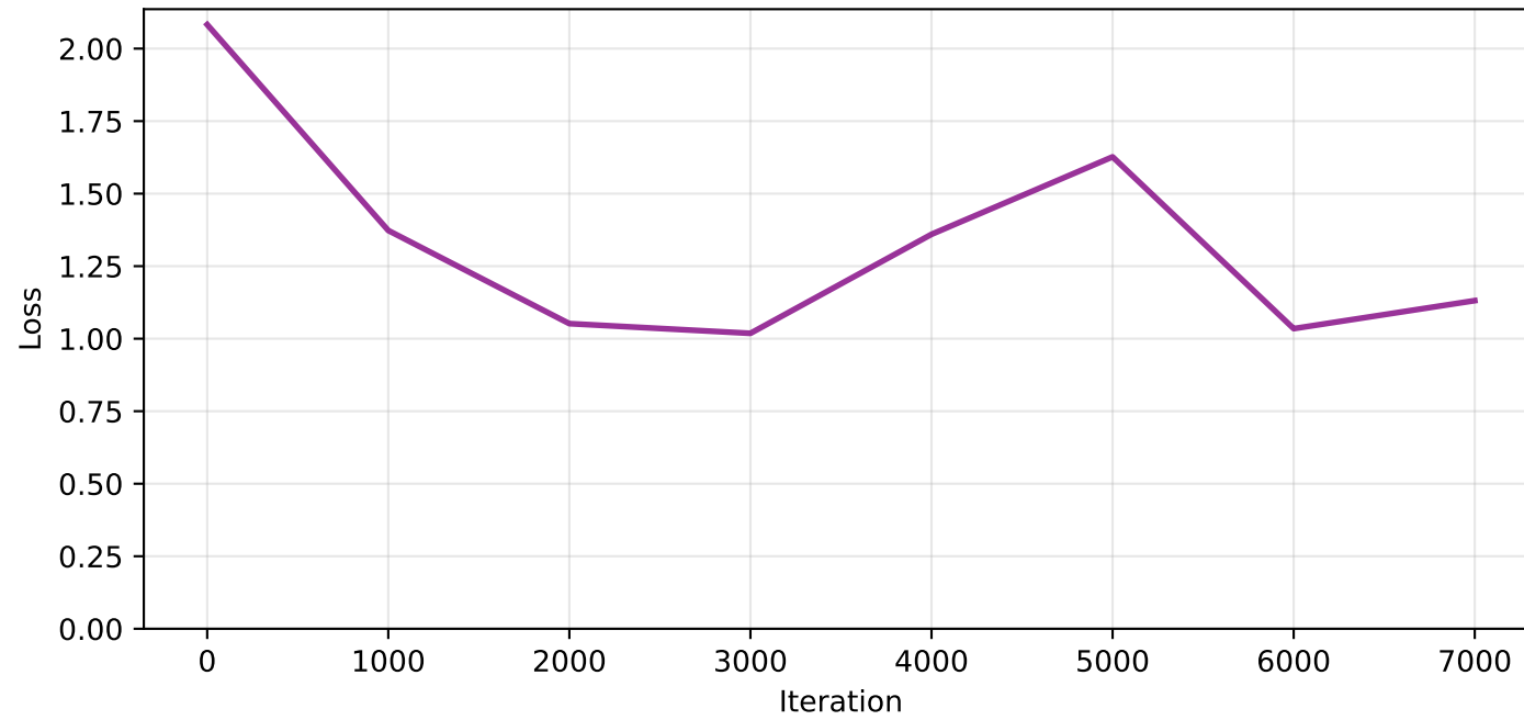
Training Loss
