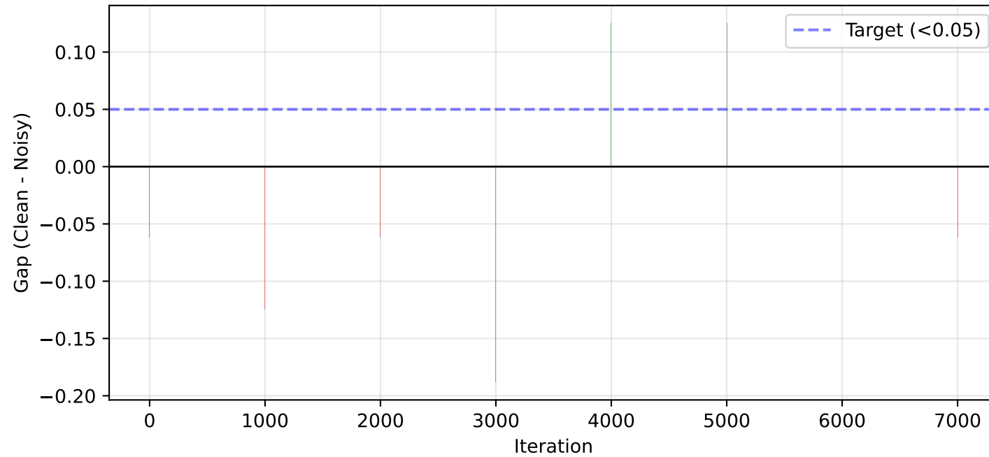
Generalization Gap
