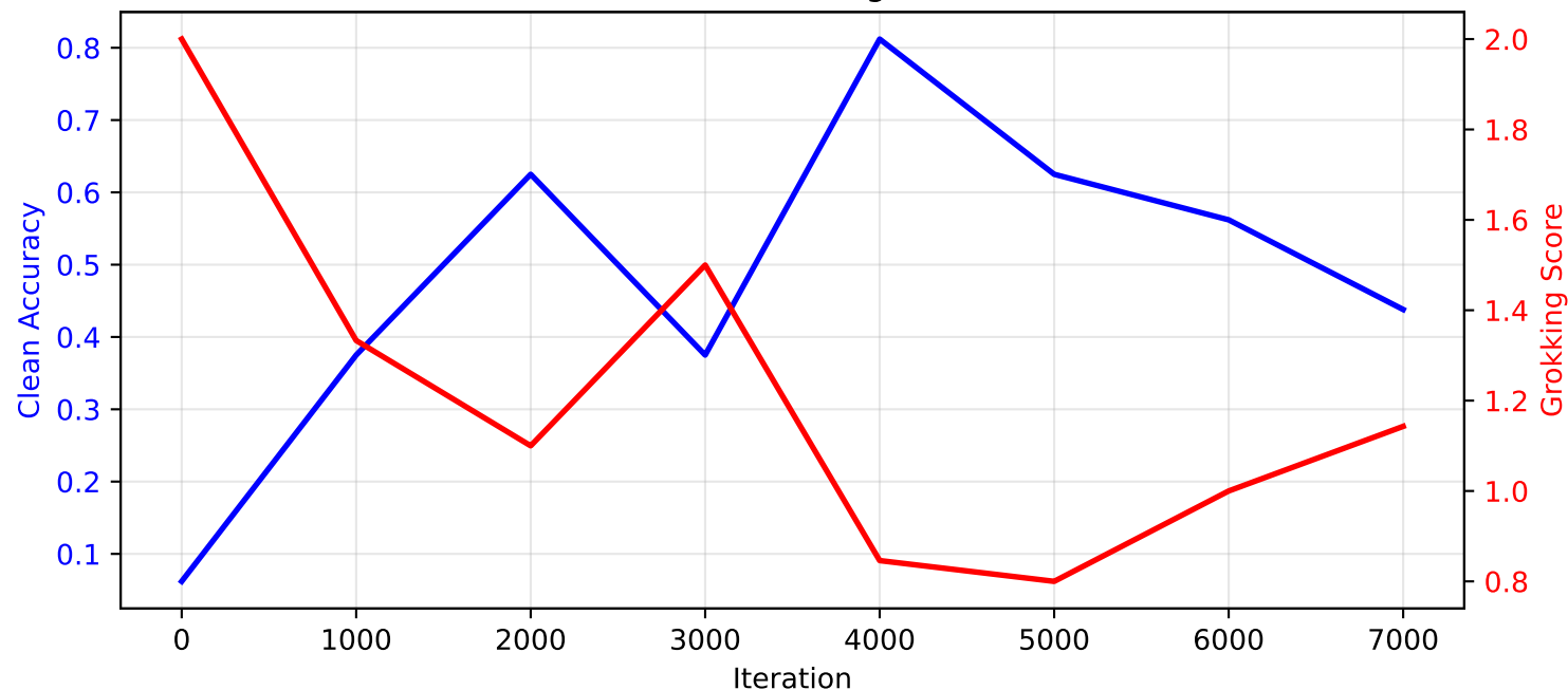
Combined Progress
