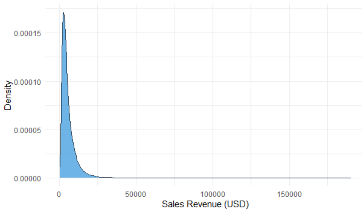
Density Plot: Sales Revenue
