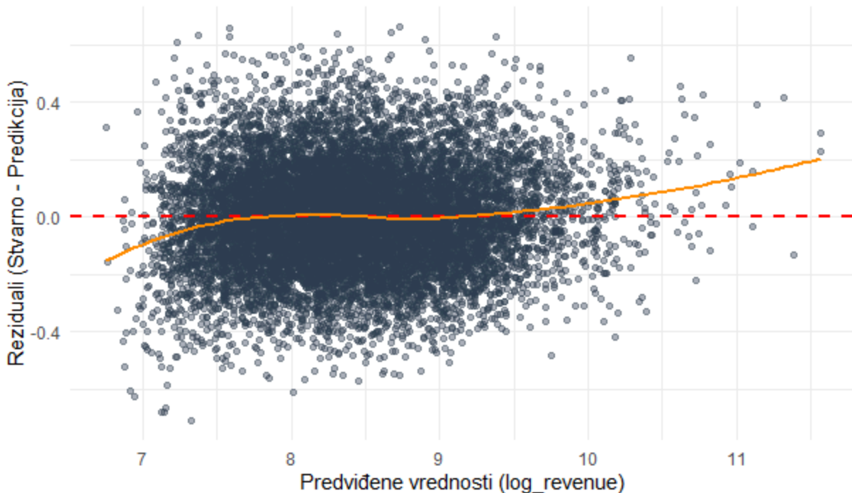
Residuals vs Predicted na test setu (GBM Model)
