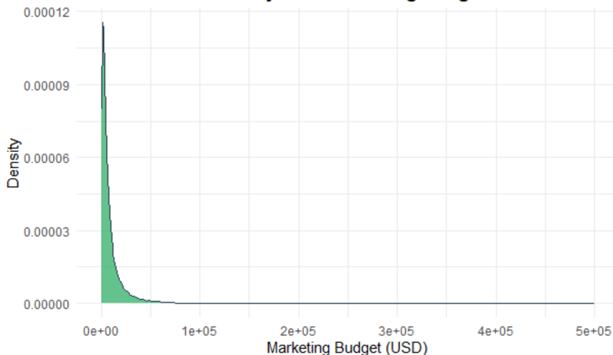
Density Plot: Marketing Budget
