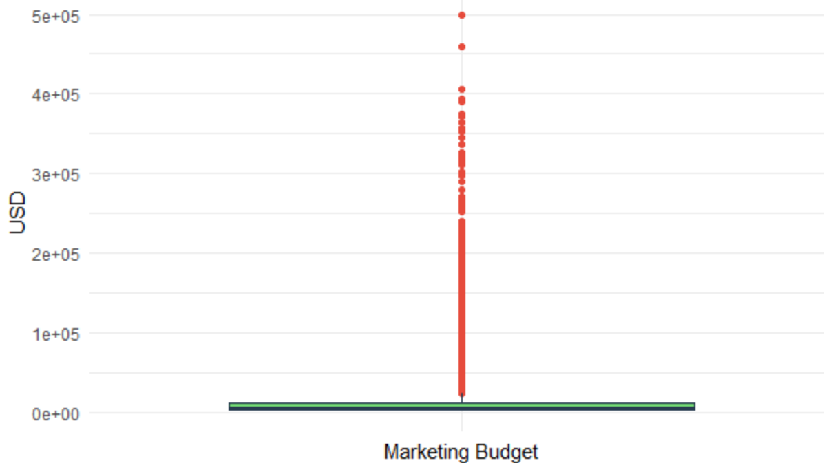
Boxplot - Marketing Budget
