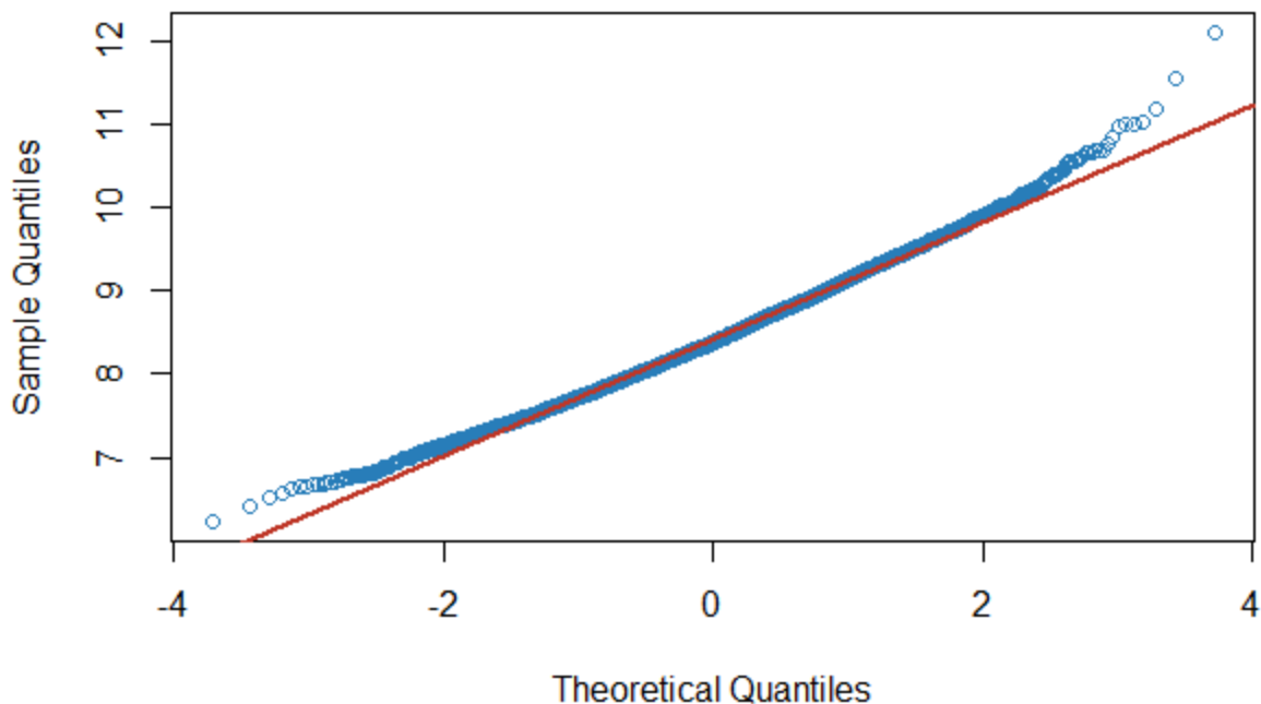
Q-Q Plot - Log-transformisani prihod
