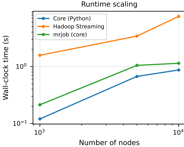
Figure 3: Wall-clock time vs. graph size (log-log). The in-memory engine and mrjob scale near-linearly in |E| ; the Streaming pipeline carries a large per-iteration constant.
