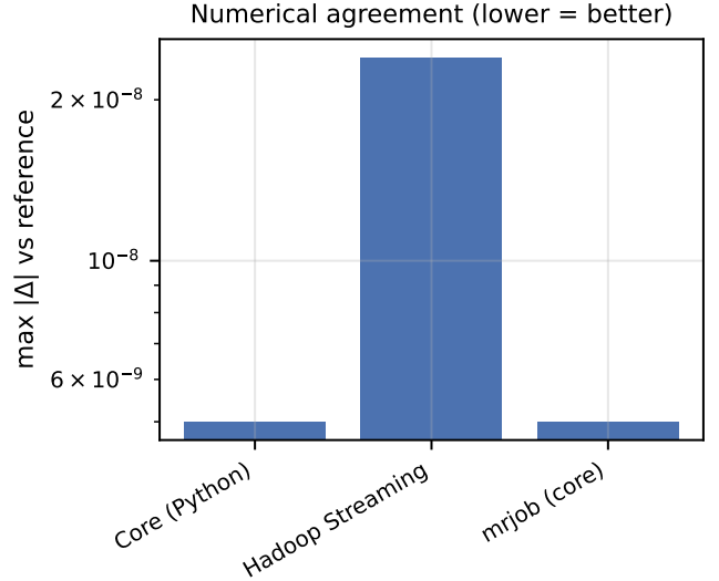
Figure 2: Maximum per-node disagreement with the reference engine (log scale, lower is better). Differences sit at the eight-decimal output-precision floor.
