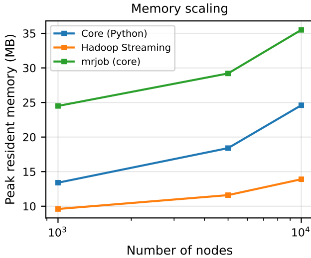
Figure 5: Peak resident memory vs. graph size. The streaming pipeline trades runtime for the smallest memory footprint.
