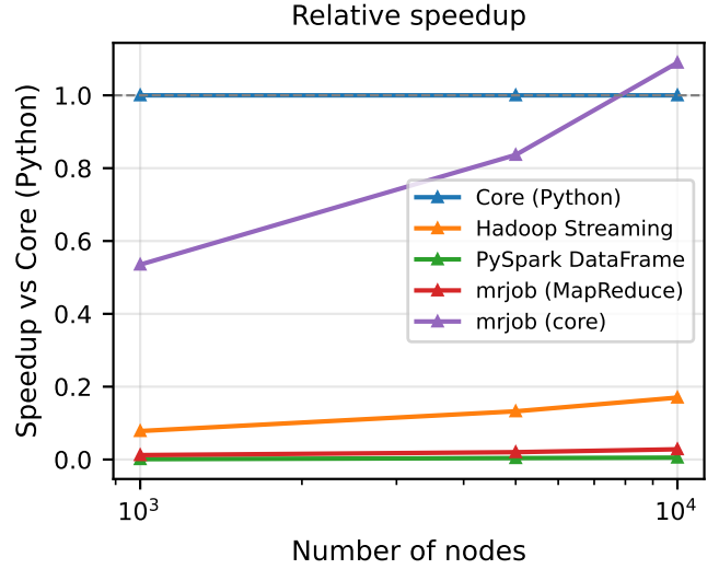
Fig. 4. Speedup relative to the pure-Python baseline. Values below 1 indicate slower execution; the framework overheads dominate at these single-node sizes.
