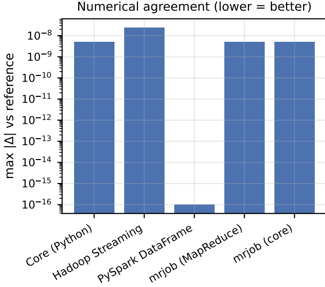
Fig. 2. Maximum per-node disagreement with the reference engine (log scale, lower is better). Differences sit at the eight-decimal output-precision floor.
