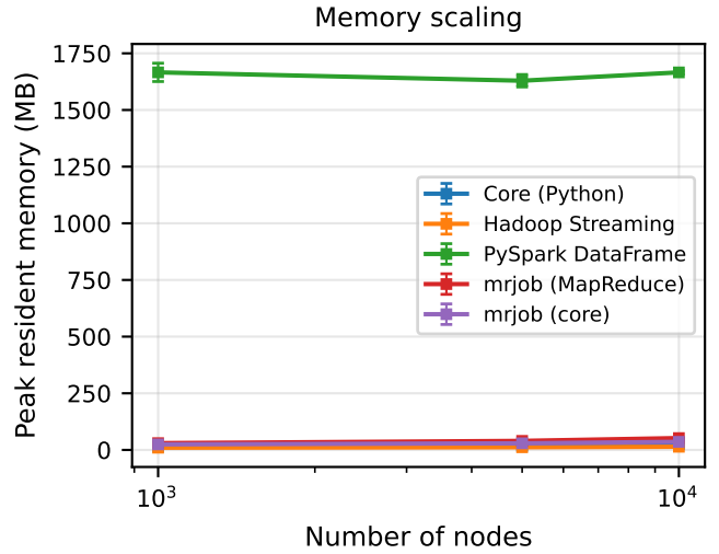
Fig. 5. Peak resident memory vs. graph size. Hadoop Streaming uses the least memory; PySpark’s \sim 1.6 GB JVM footprint is two orders of magnitude larger than the Python engines at these scales.
