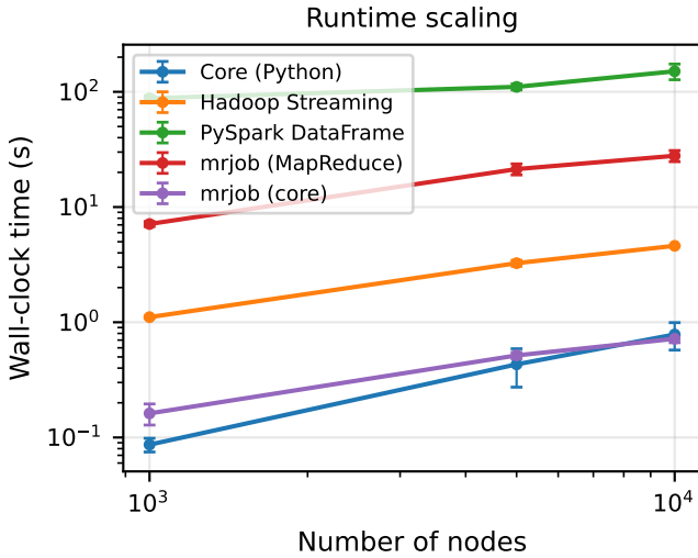
Fig. 3. Wall-clock time vs. graph size (log-log, mean of three runs with standard-deviation error bars). The in-memory engines scale near-linearly in |E| ; the single-pass Streaming, mrjob MapReduce, and PySpark DataFrame engines carry large per-iteration constants (PySpark’s curve sits highest).
