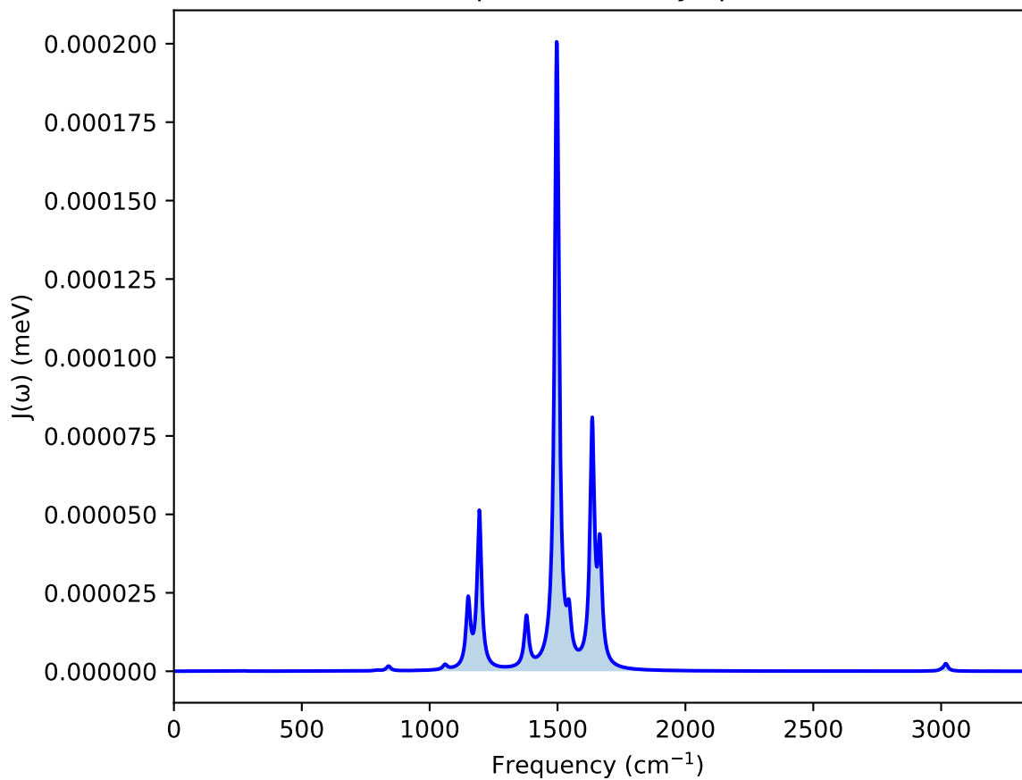
Broadened Spectral Density ( \gamma = 10 \text{ cm}^{-1} )
