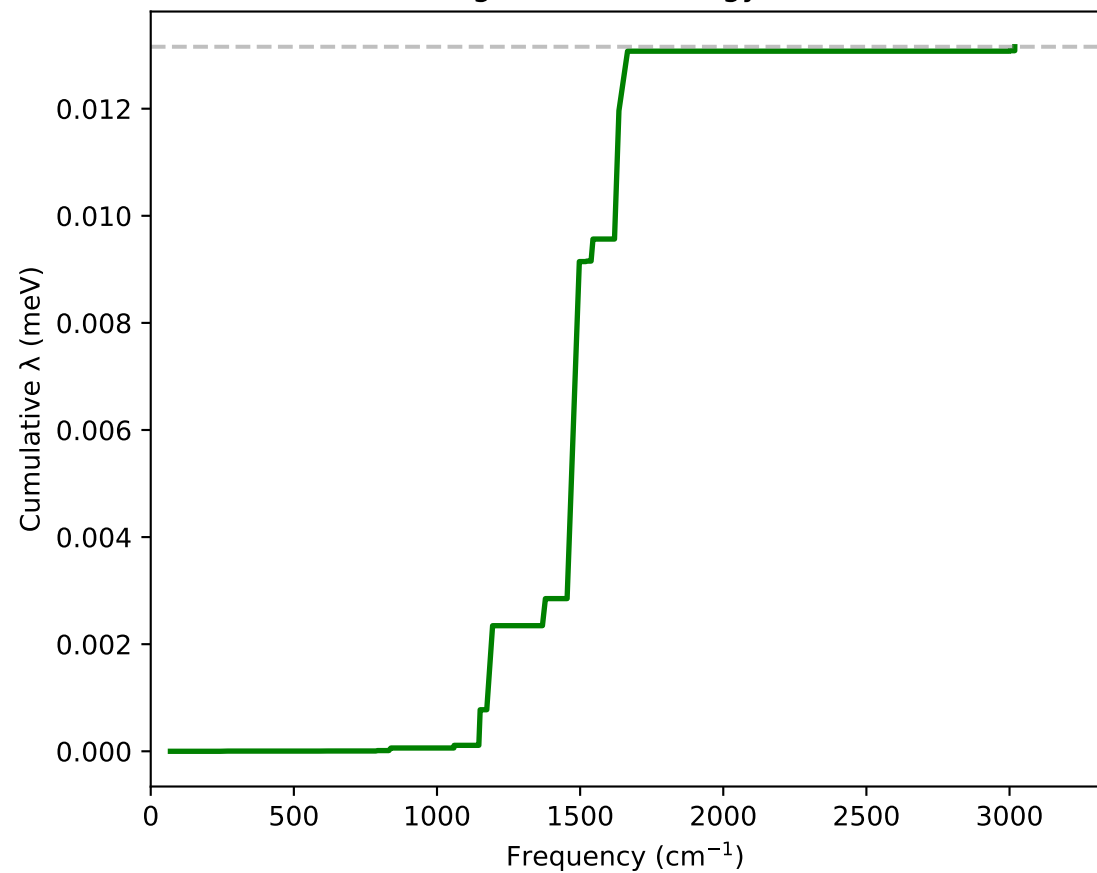
Cumulative Reorganization Energy (Total: 0.01 meV)
