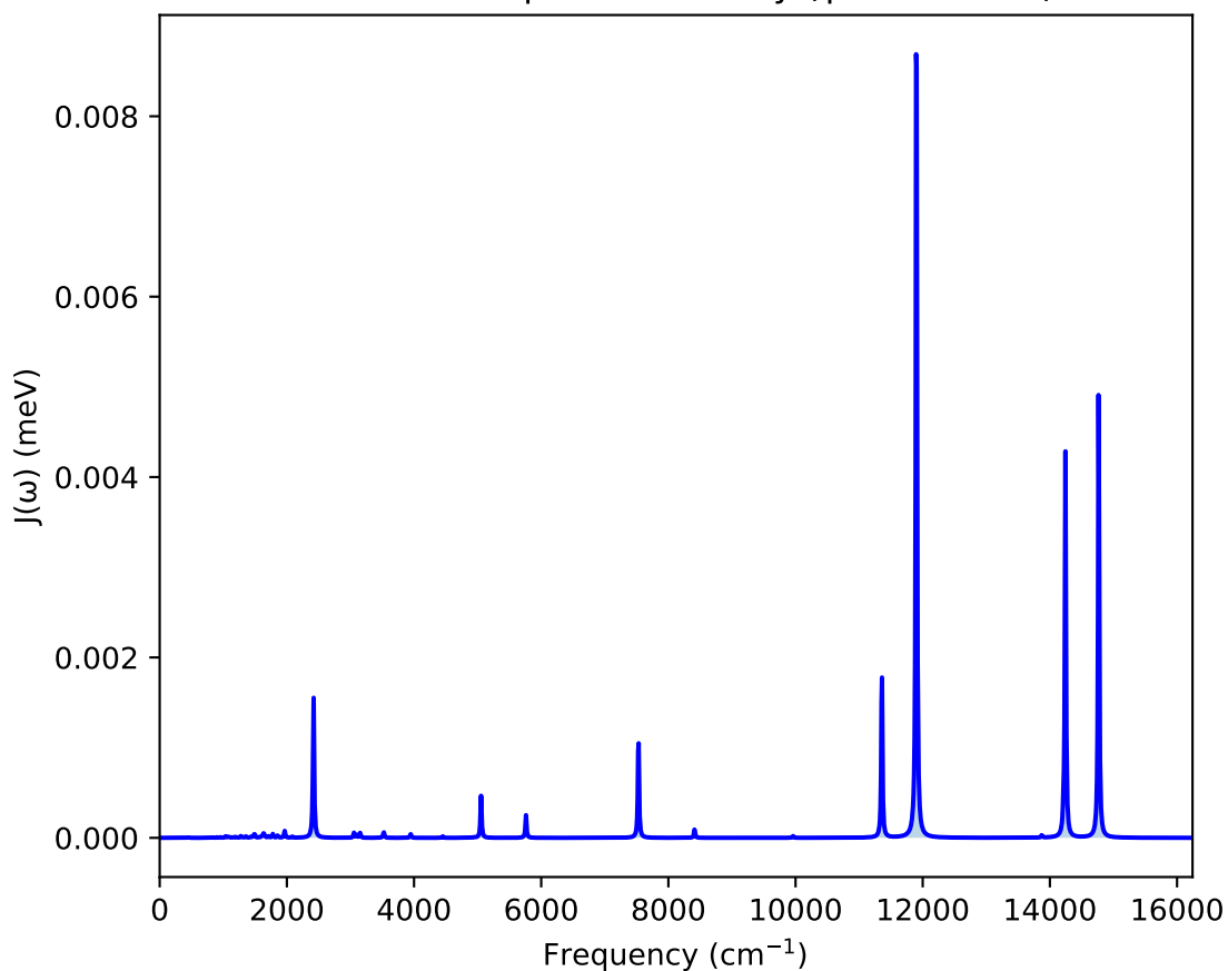
Broadened Spectral Density ( \gamma = 10 \text{ cm}^{-1} )
