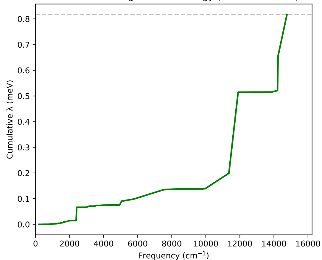
Cumulative Reorganization Energy (Total: 0.82 meV)
