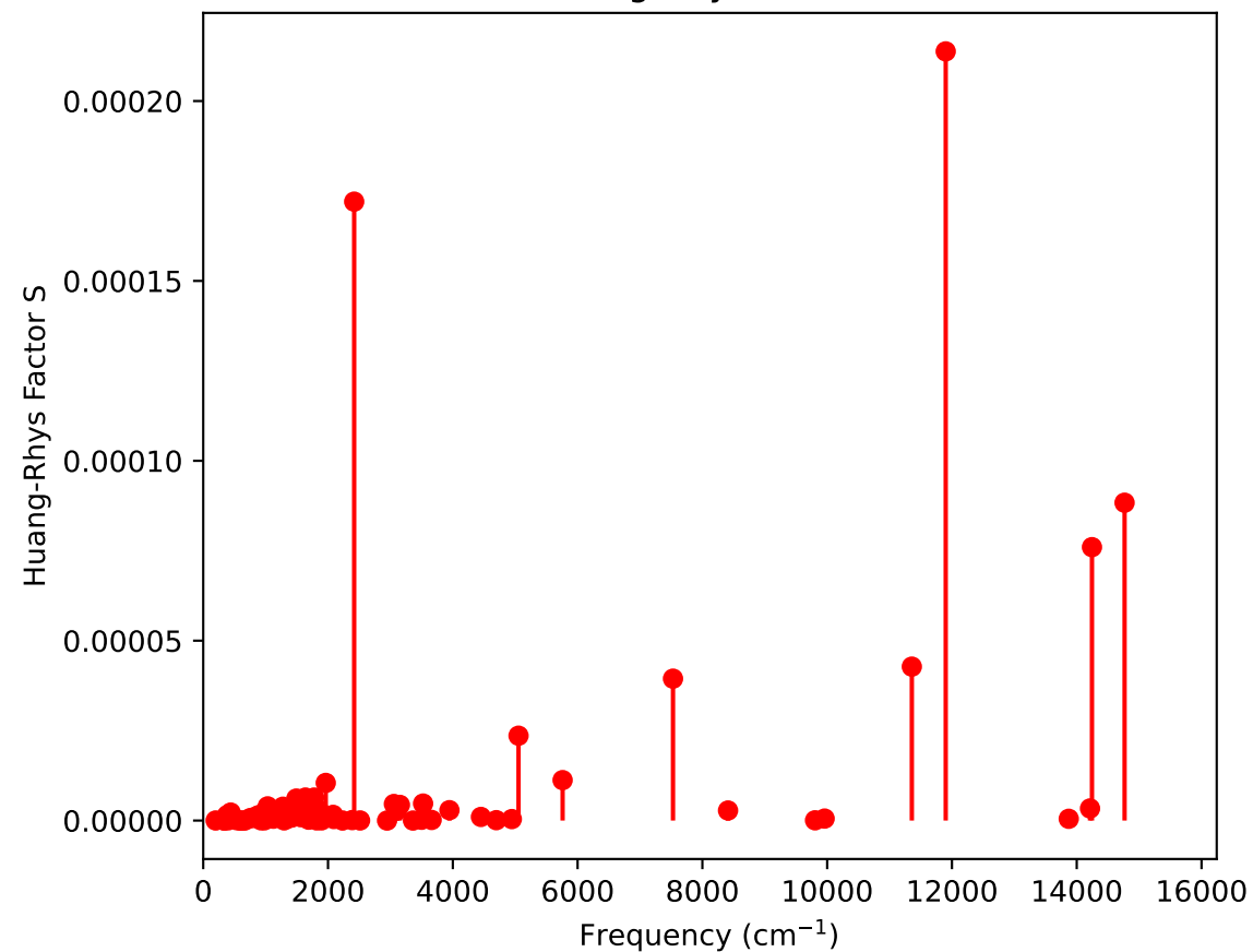
Huang-Rhys Factors
