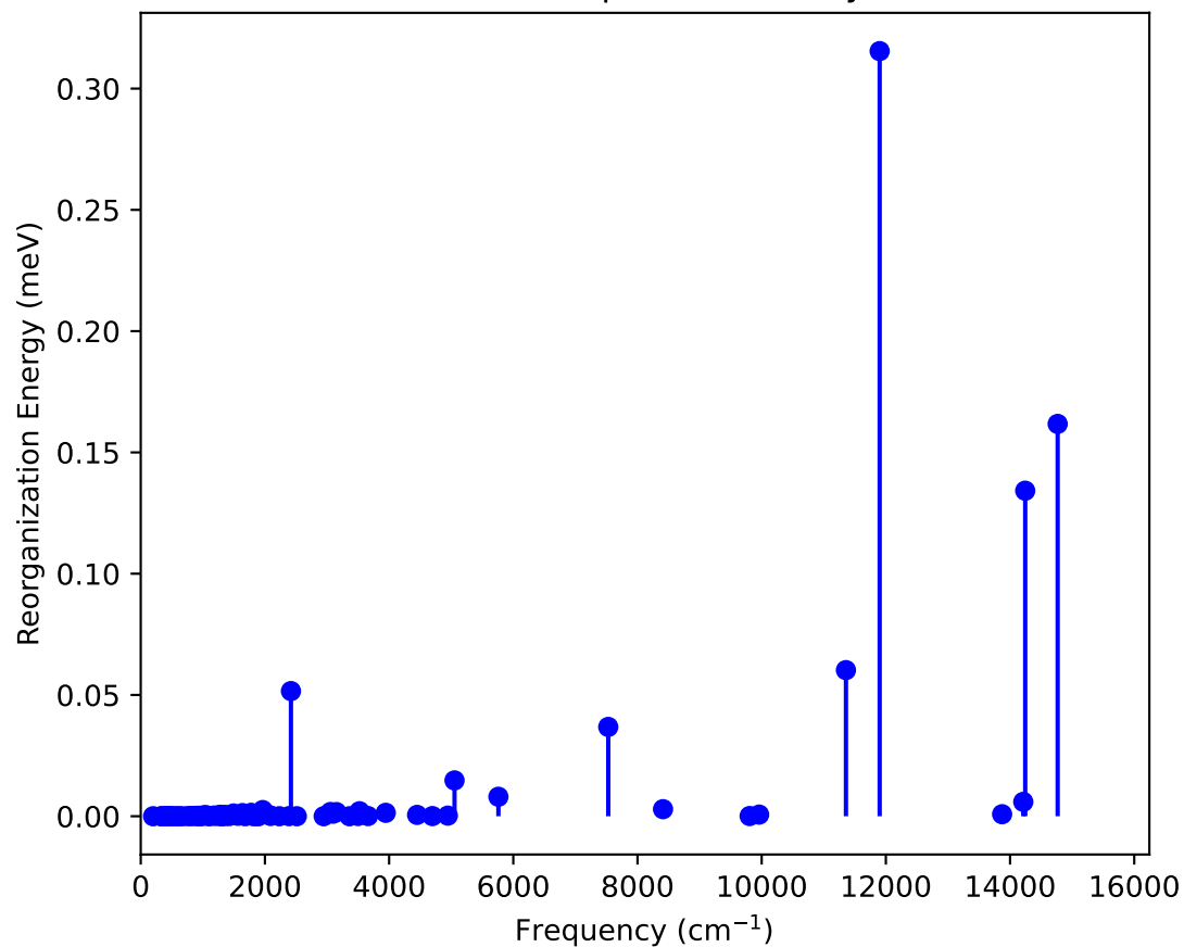
Discrete Spectral Density
