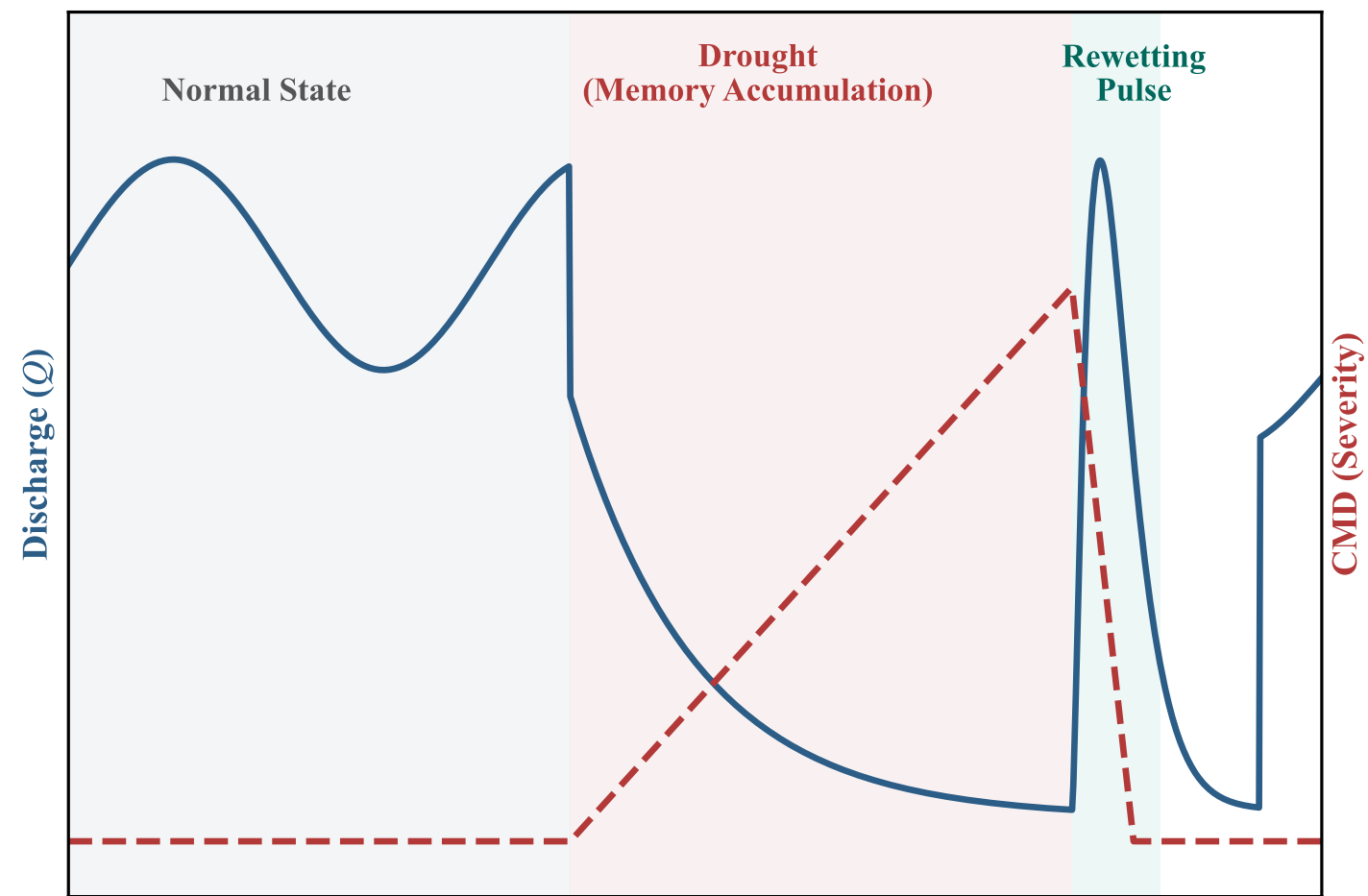
(a) Hydrological States & Memory Effect
