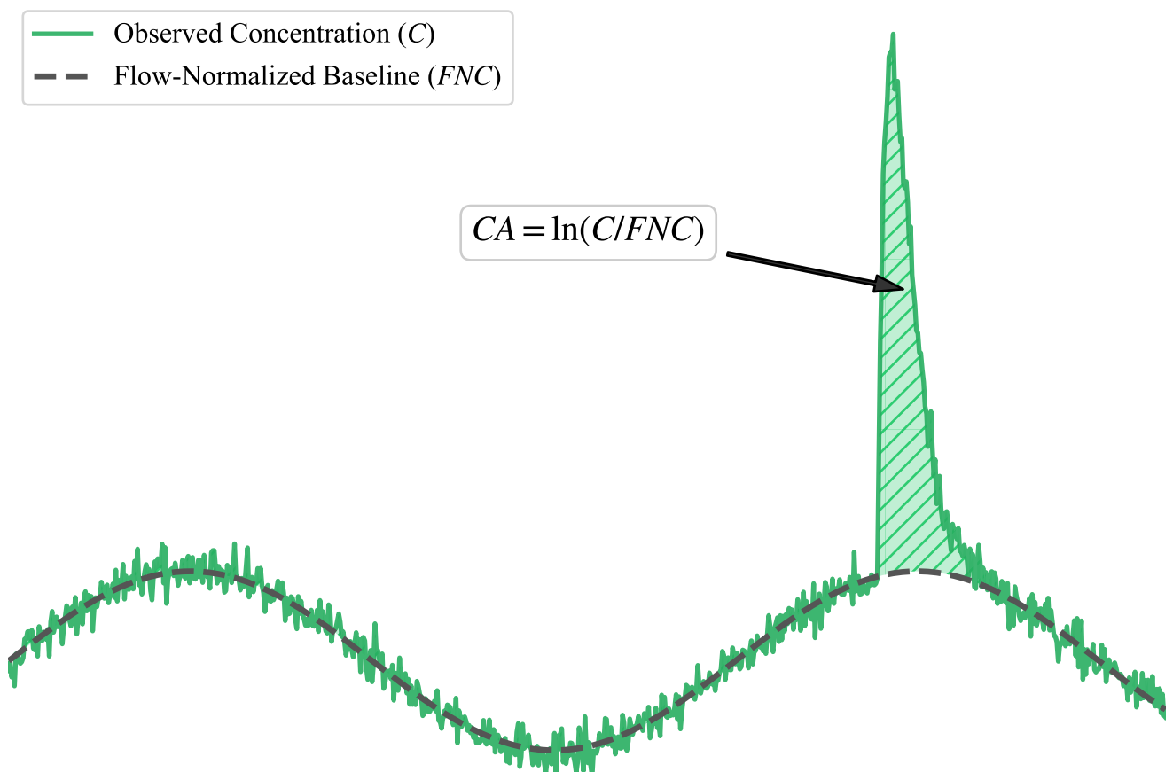
(b) Concentration Anomaly (CA) Extraction
