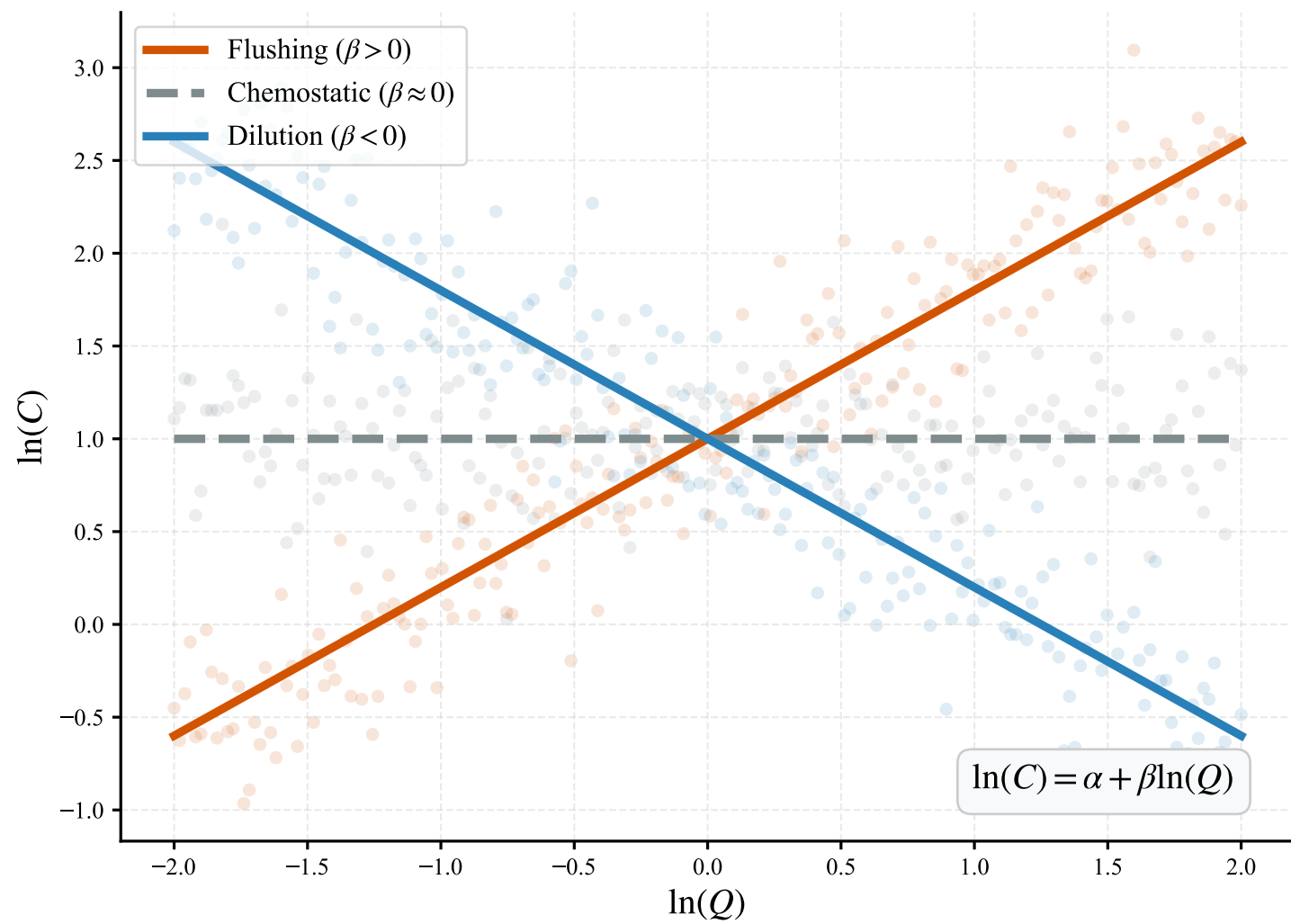
(c) State-Dependent c-Q Slopes ( \beta )
