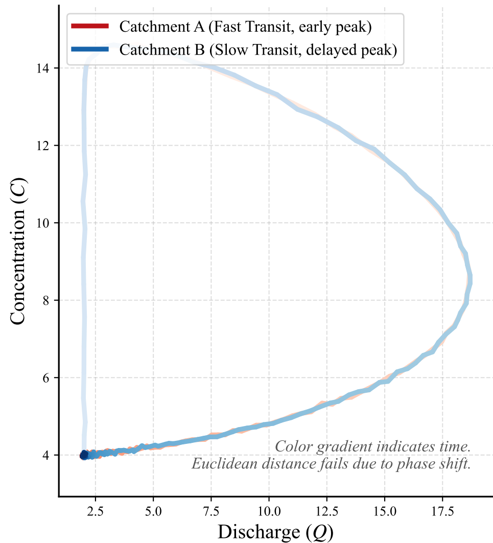
(a) Chaotic Phase Space (Unaligned)
