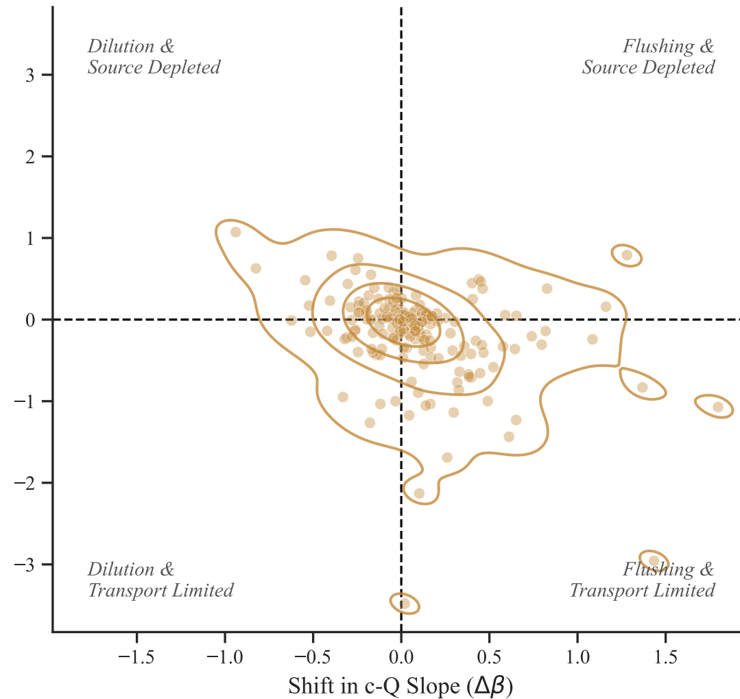
PO4P Regime Shifts
