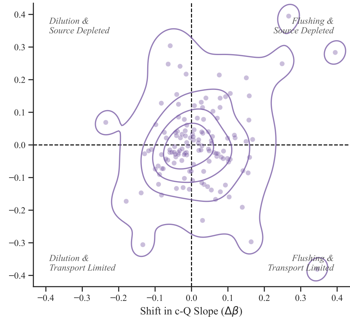
DOC Regime Shifts
