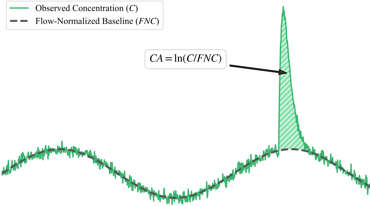
(b) Concentration Anomaly (CA) Extraction
