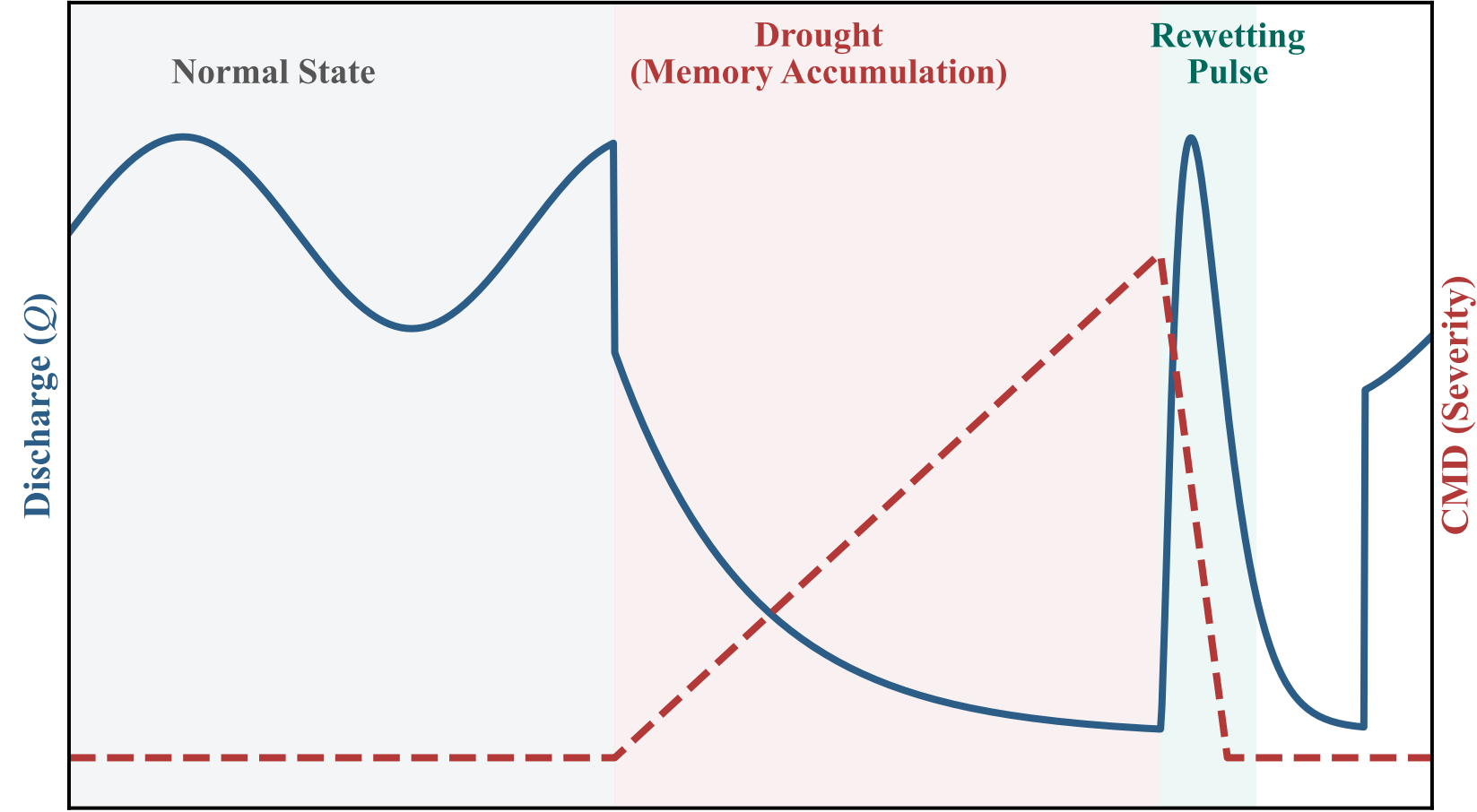
(a) Hydrological States & Memory Effect
