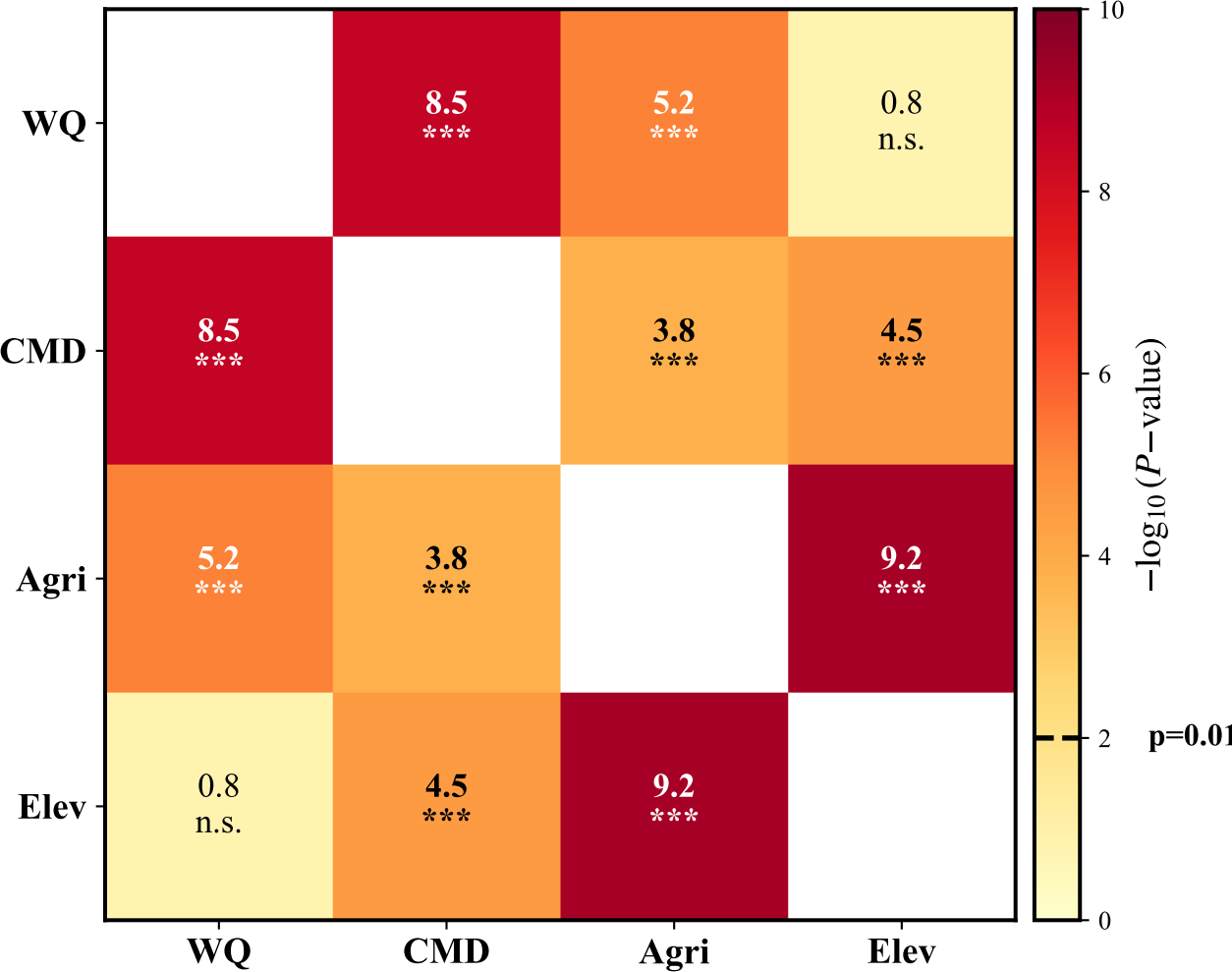
(c) Momentary Conditional Independence Matrix ( -\log_{10}(P) )
