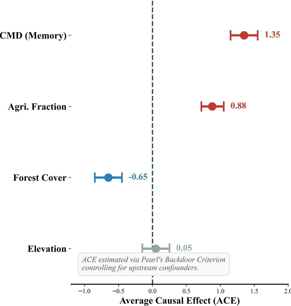
(b) Backdoor-Adjusted Causal Effects
