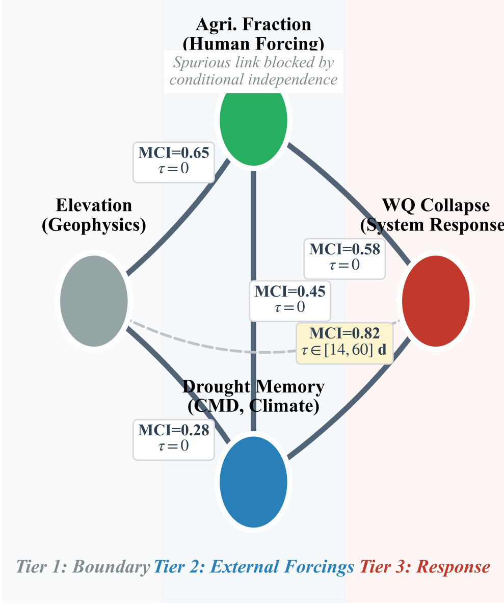
(a) PCMCI+ Spatiotemporal Causal DAG
