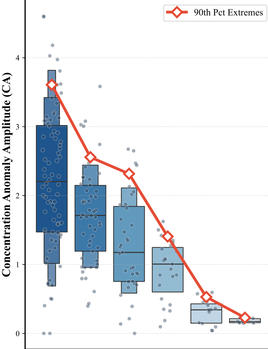
(b) Signal Modulation by Topology Depth
