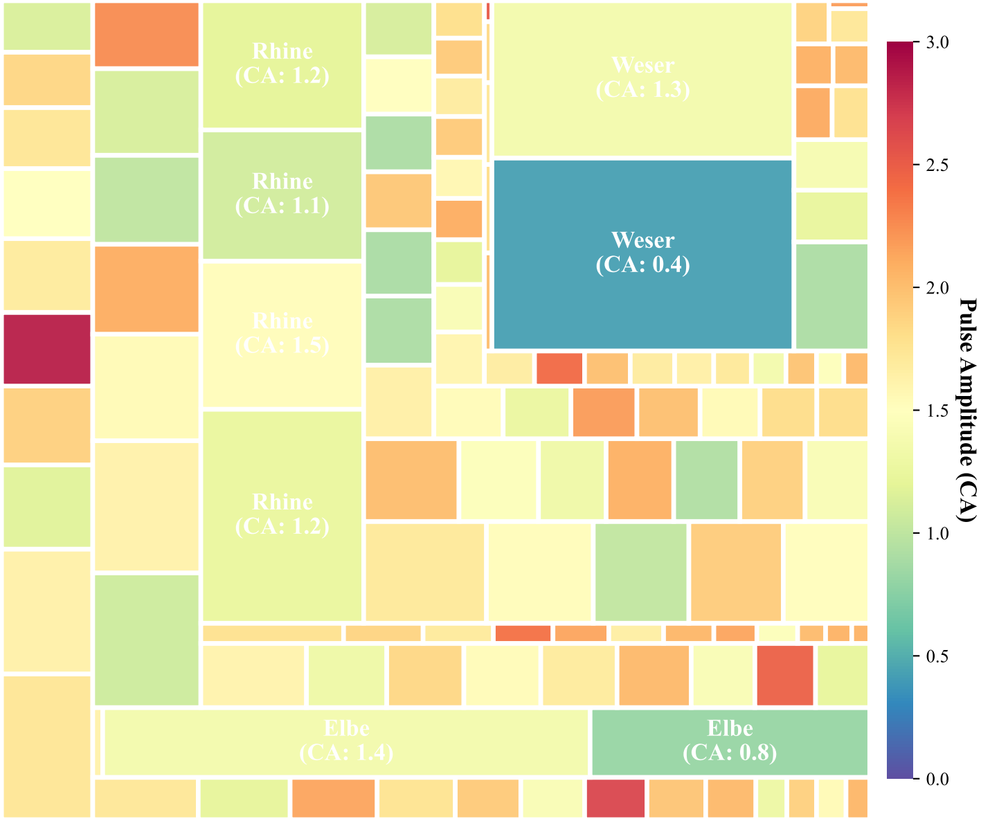
(a) Spatial Mosaic of Vulnerability Nestedness
