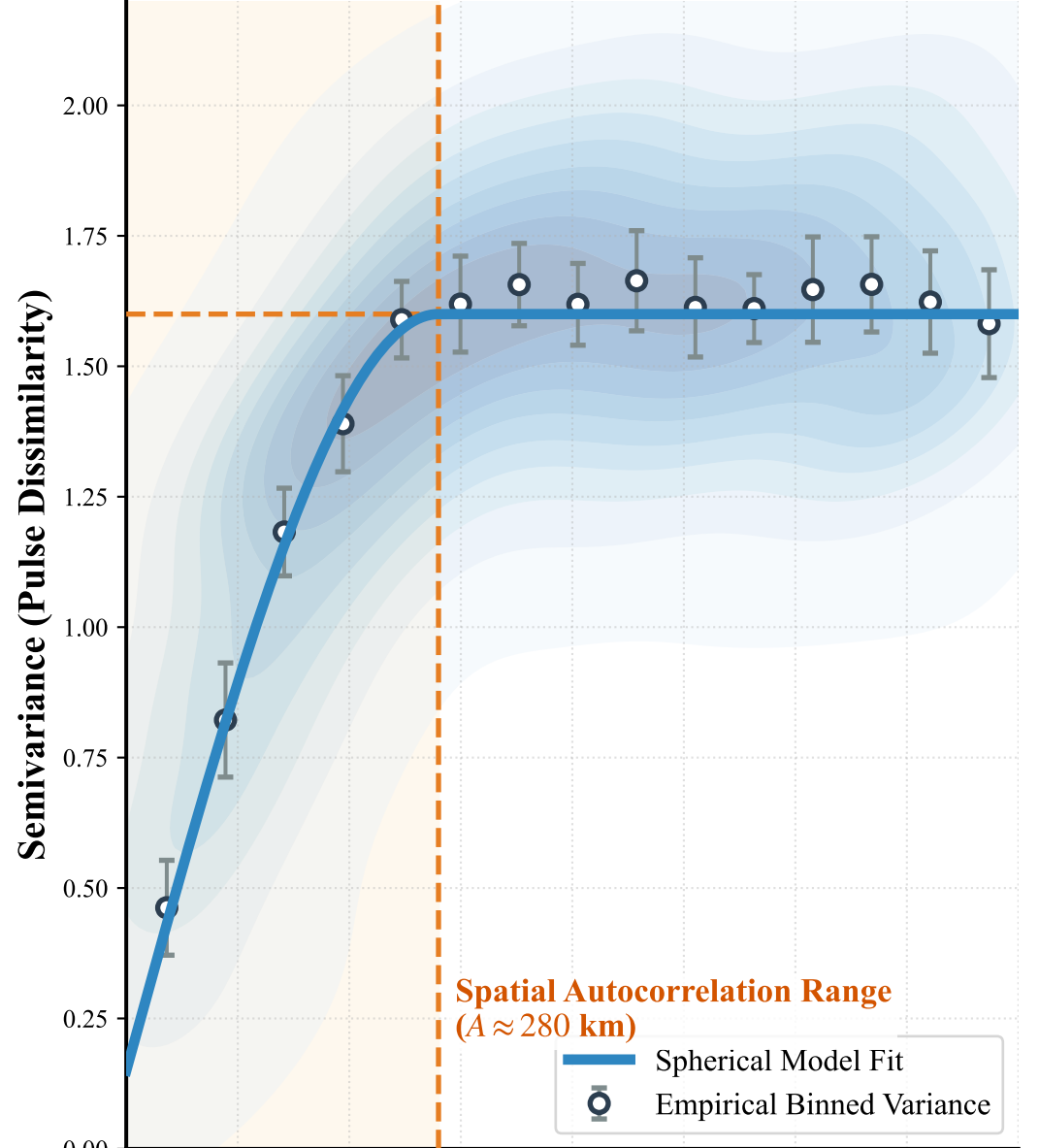
(c) Spatial Distance Decay (Variogram)
