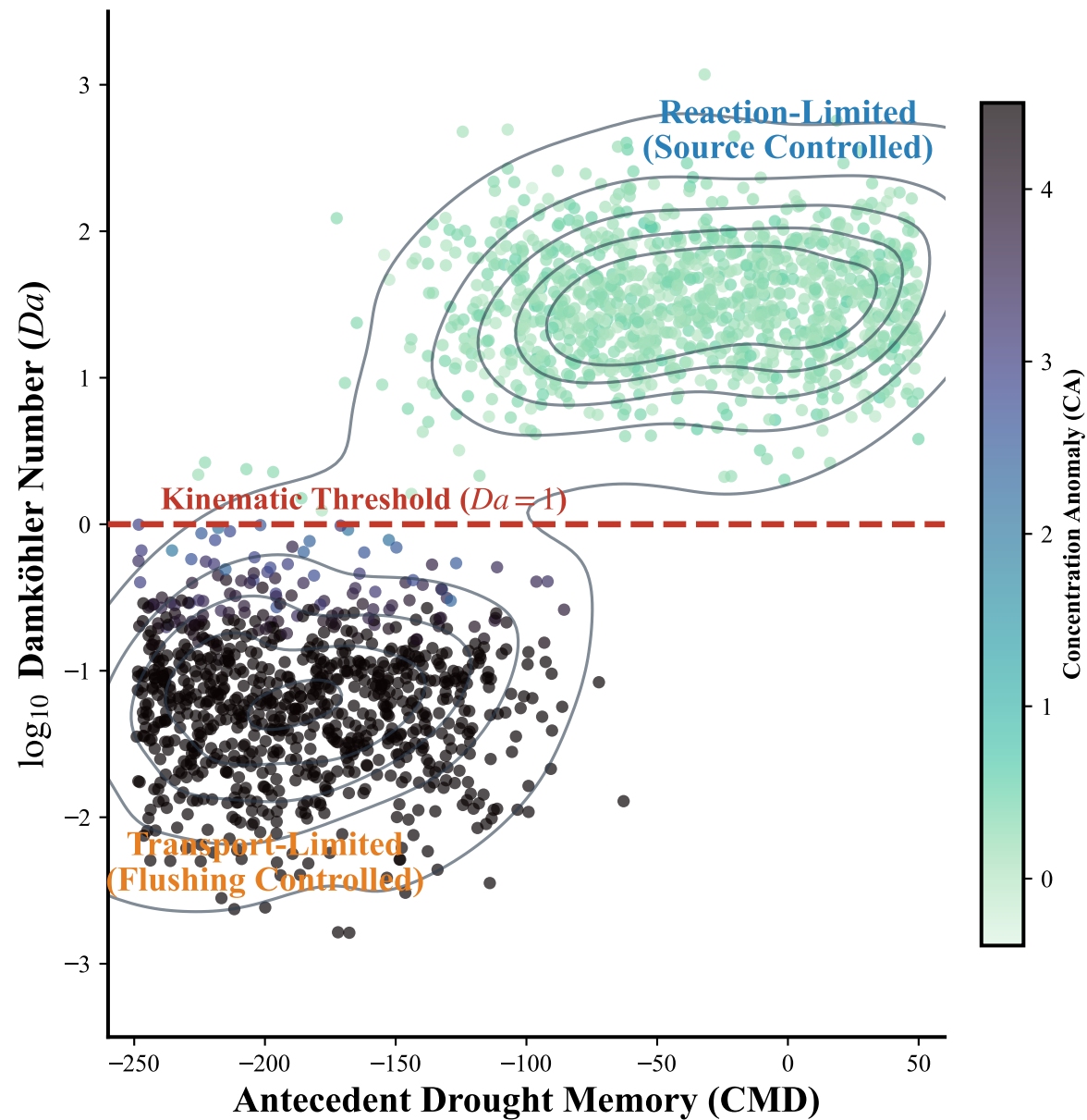
(a) Thermodynamic Phase Space Collapse
