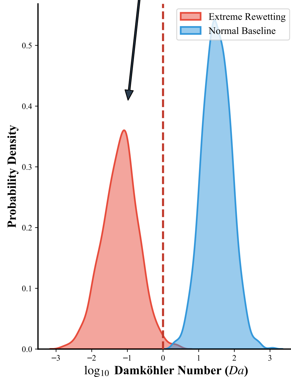
(b) Probability Drift of Transport State
