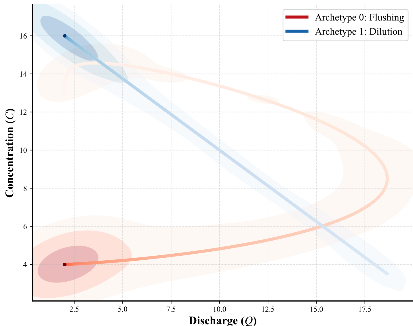
(c) True Archetypes Extracted by Constrained DTW
