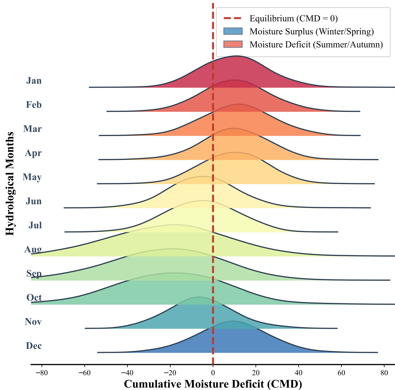
(a) Seasonal Evolution of Drought Memory
