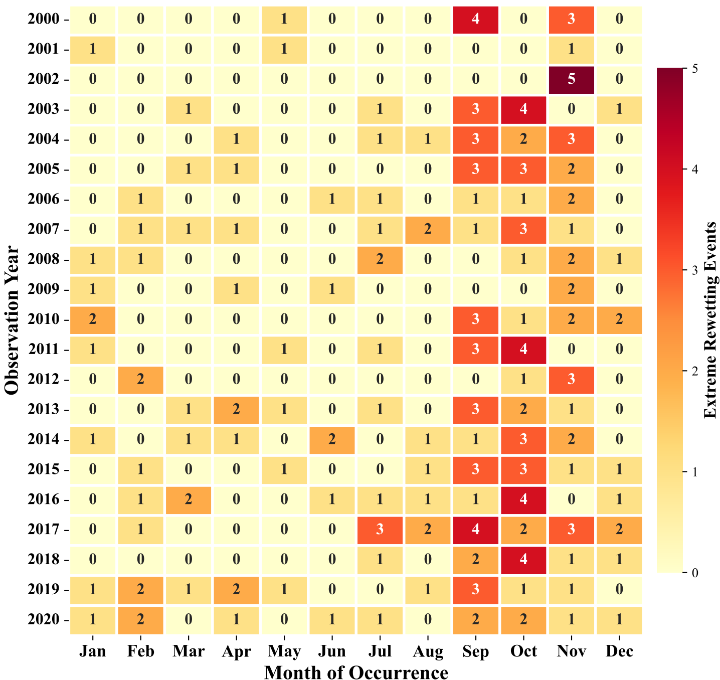
(b) Decadal Intensification of Compounding Extremes
