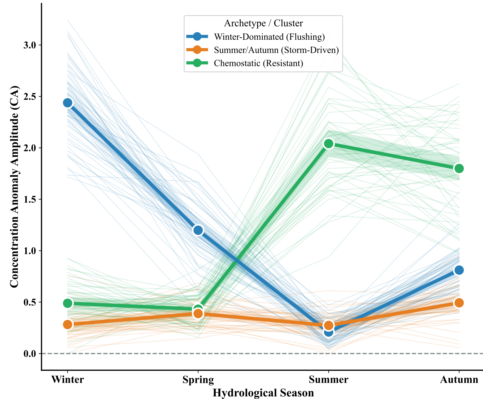
(c) Catchment Longitudinal Trajectories
