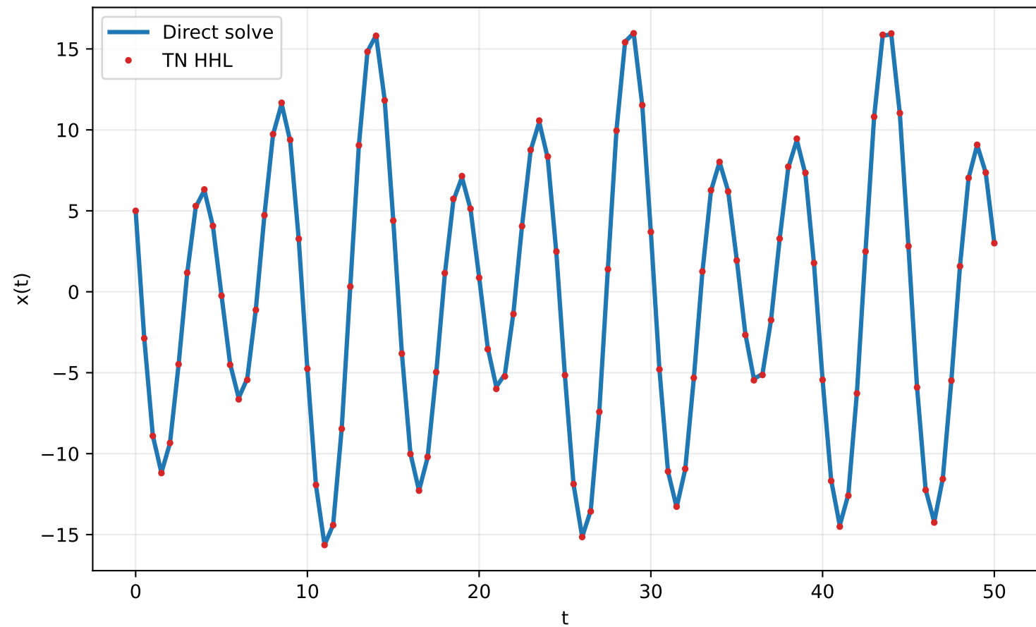
Forced harmonic oscillator (100 intervals, 99 interior unknowns)
