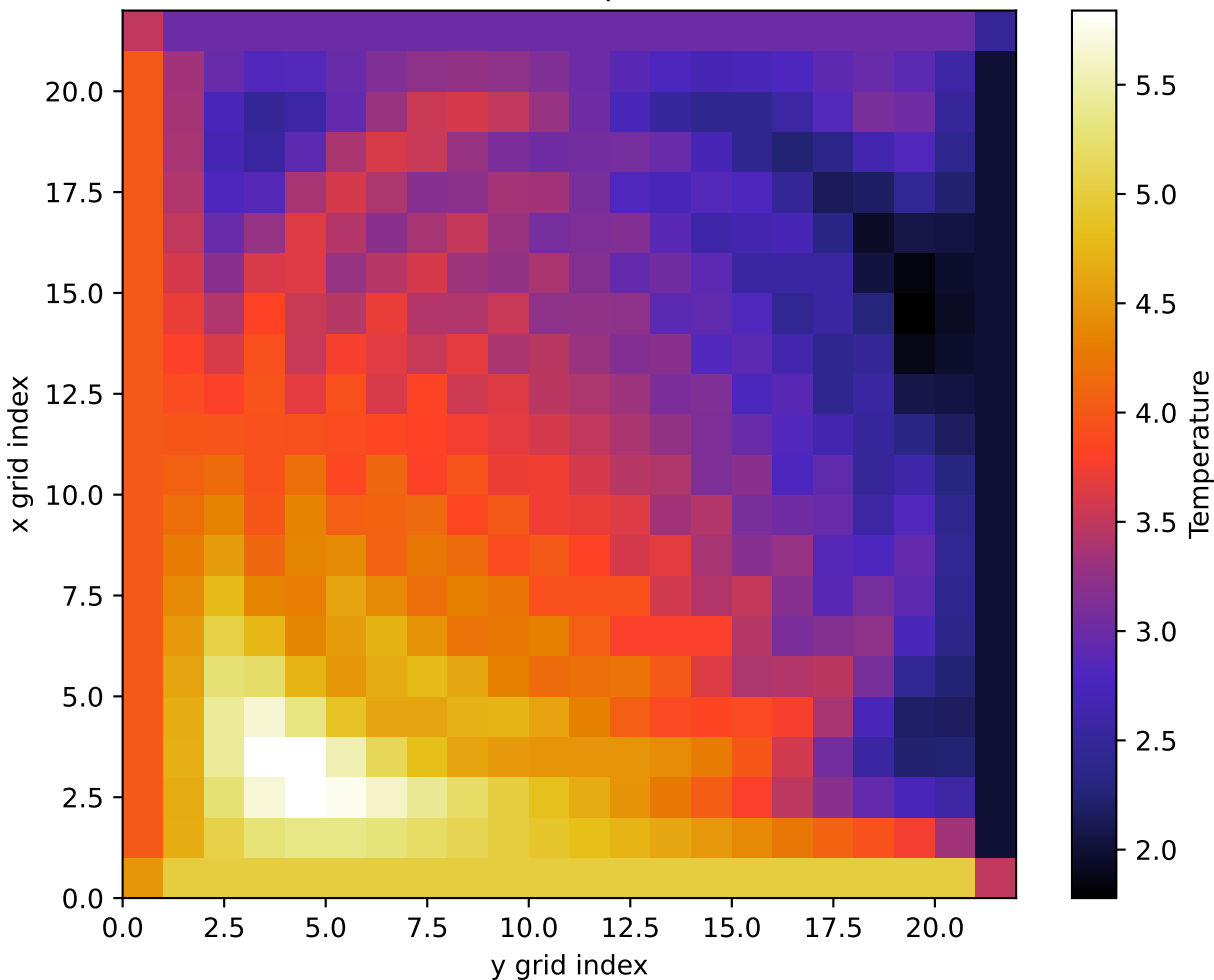
TN HHL heat solution with prescribed boundaries
