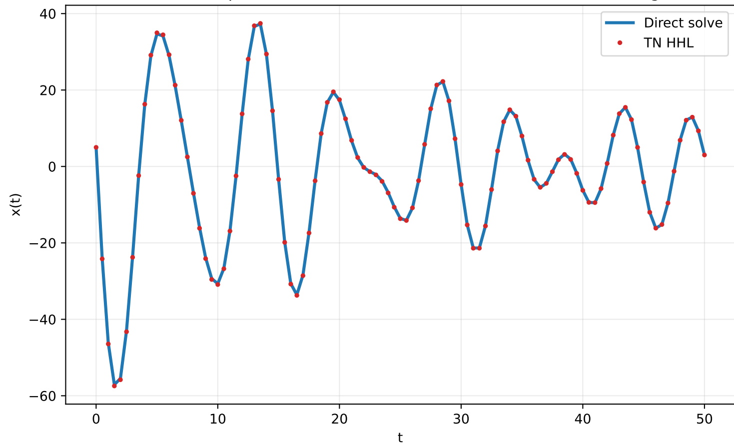
Forced damped oscillator (198-dimensional Hermitian embedding)
