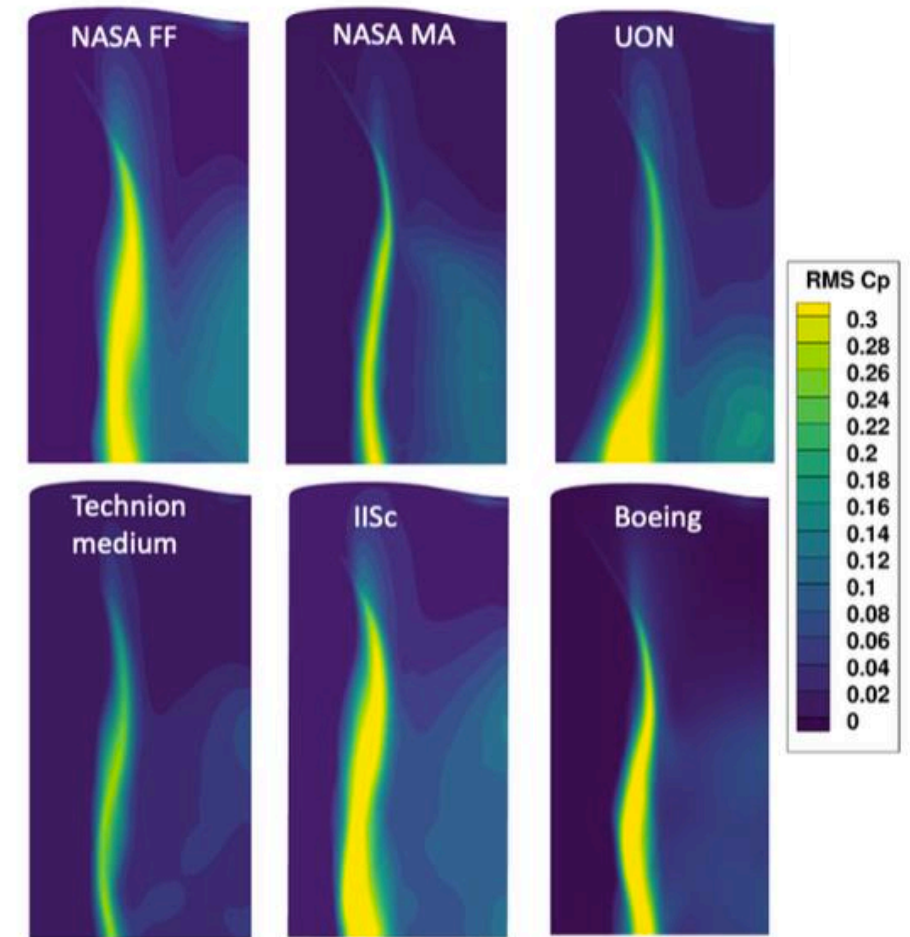
AePW-III data
