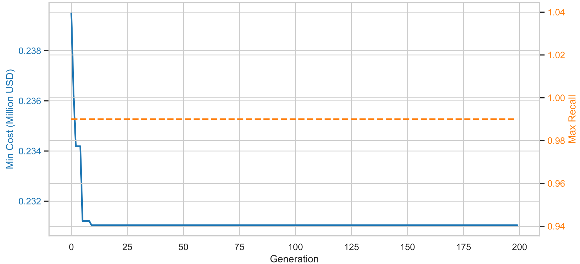
Optimization Convergence
