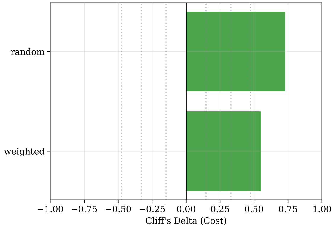
(a) Effect Size: Cost (Positive = NSGA-III Better)
