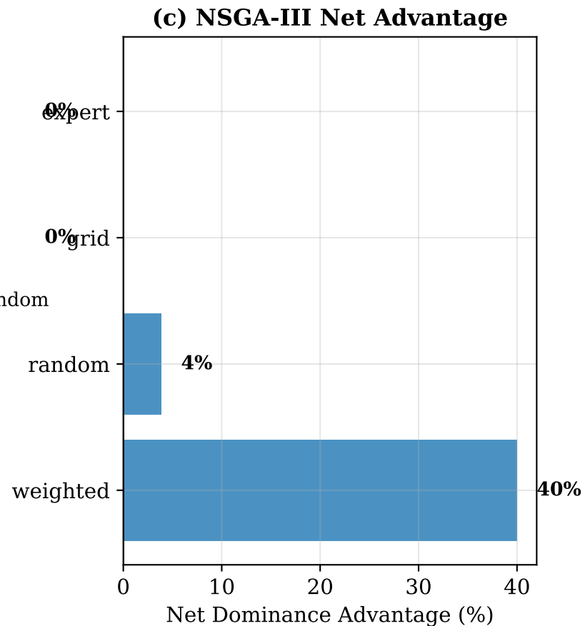
Figure 2: NSGA-III Dominance and Contribution Analysis
