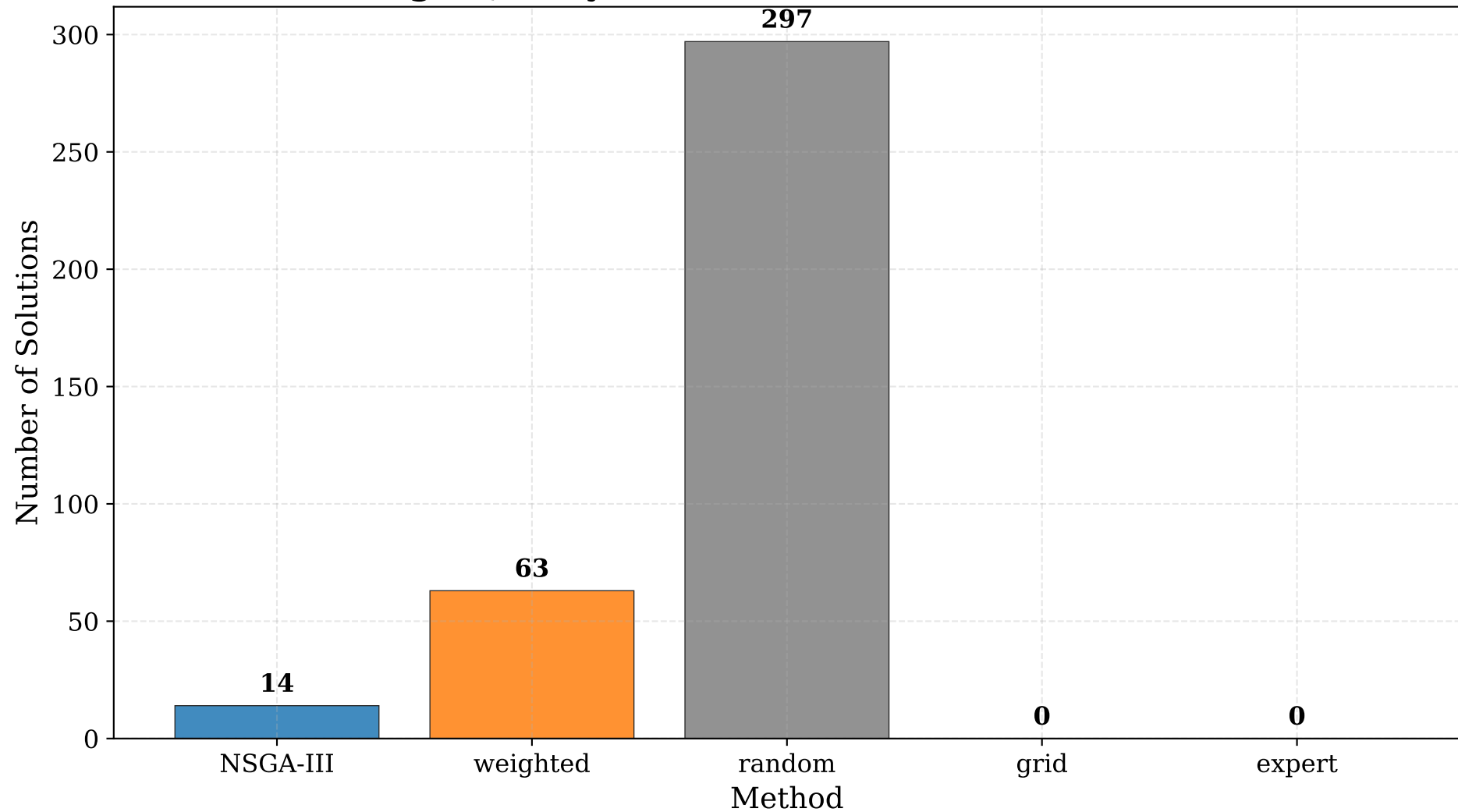
High-Quality Solutions Count (Recall \geq 0.95 )
