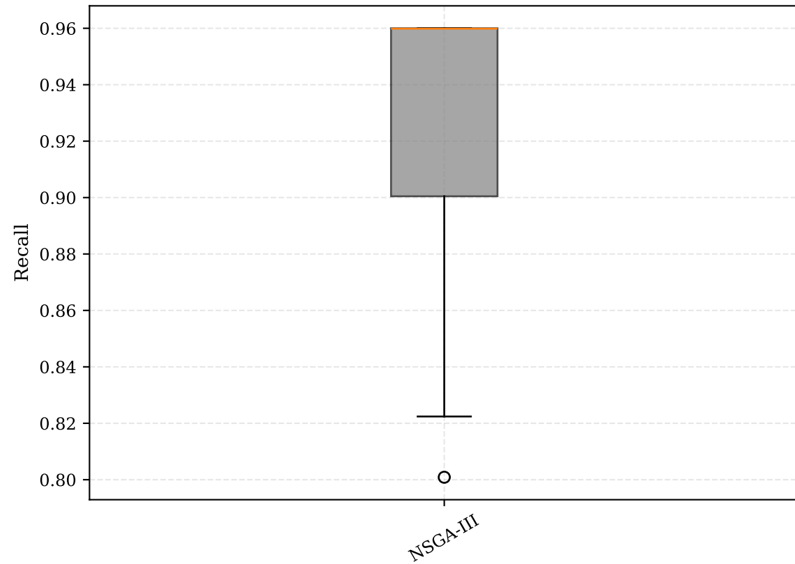
(b) Recall Distribution
