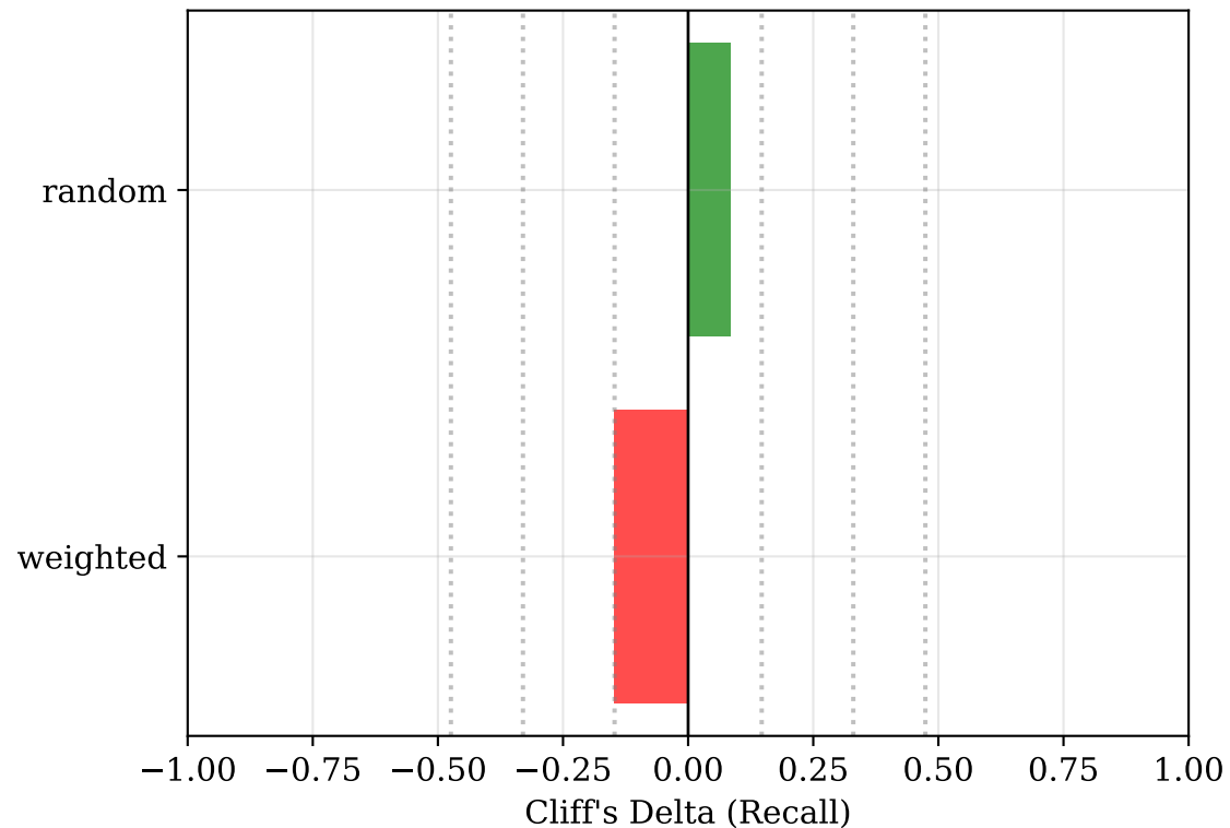
(b) Effect Size: Recall (Positive = NSGA-III Better)
