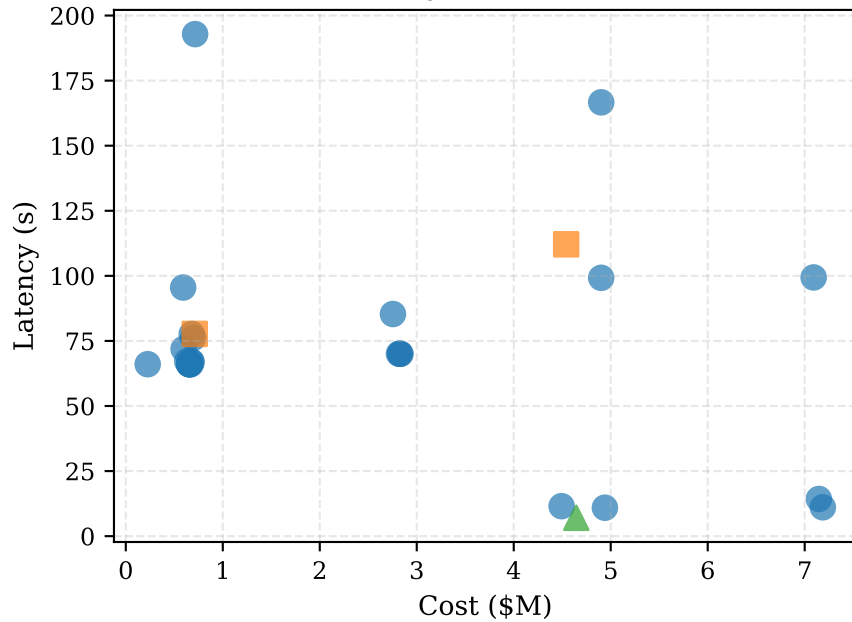
(b) Latency (s) vs Cost ($M)
