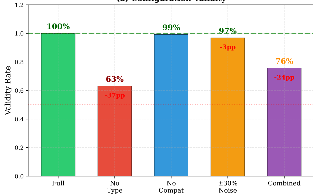
(a) Configuration Validity
