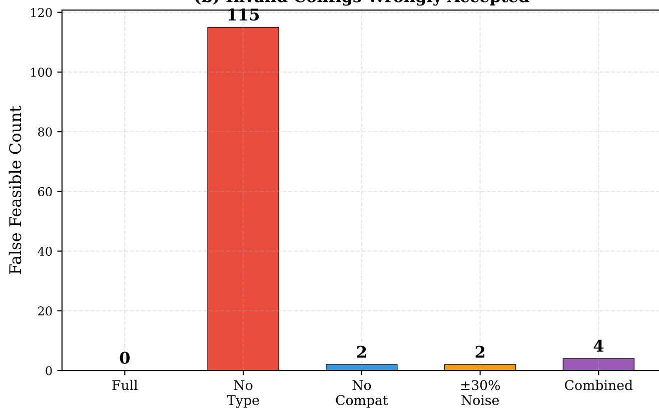
(b) Invalid Configs Wrongly Accepted
