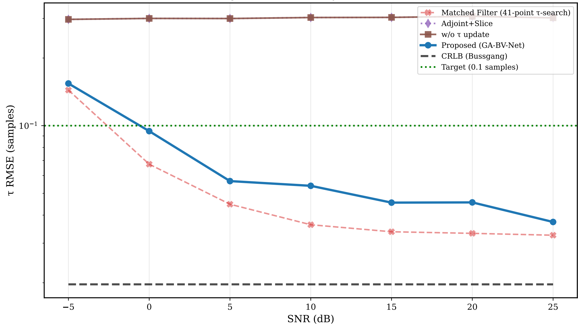
Sensing Performance: Delay Estimation Error
