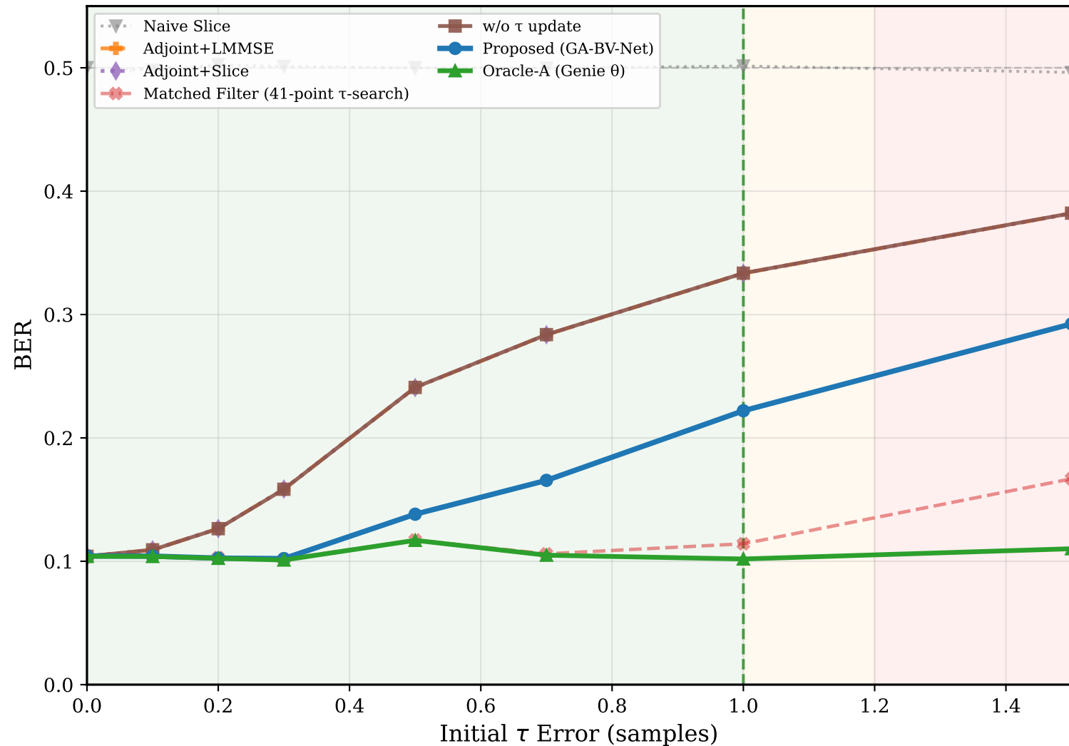
(a) The Cliff: Detection Robustness
