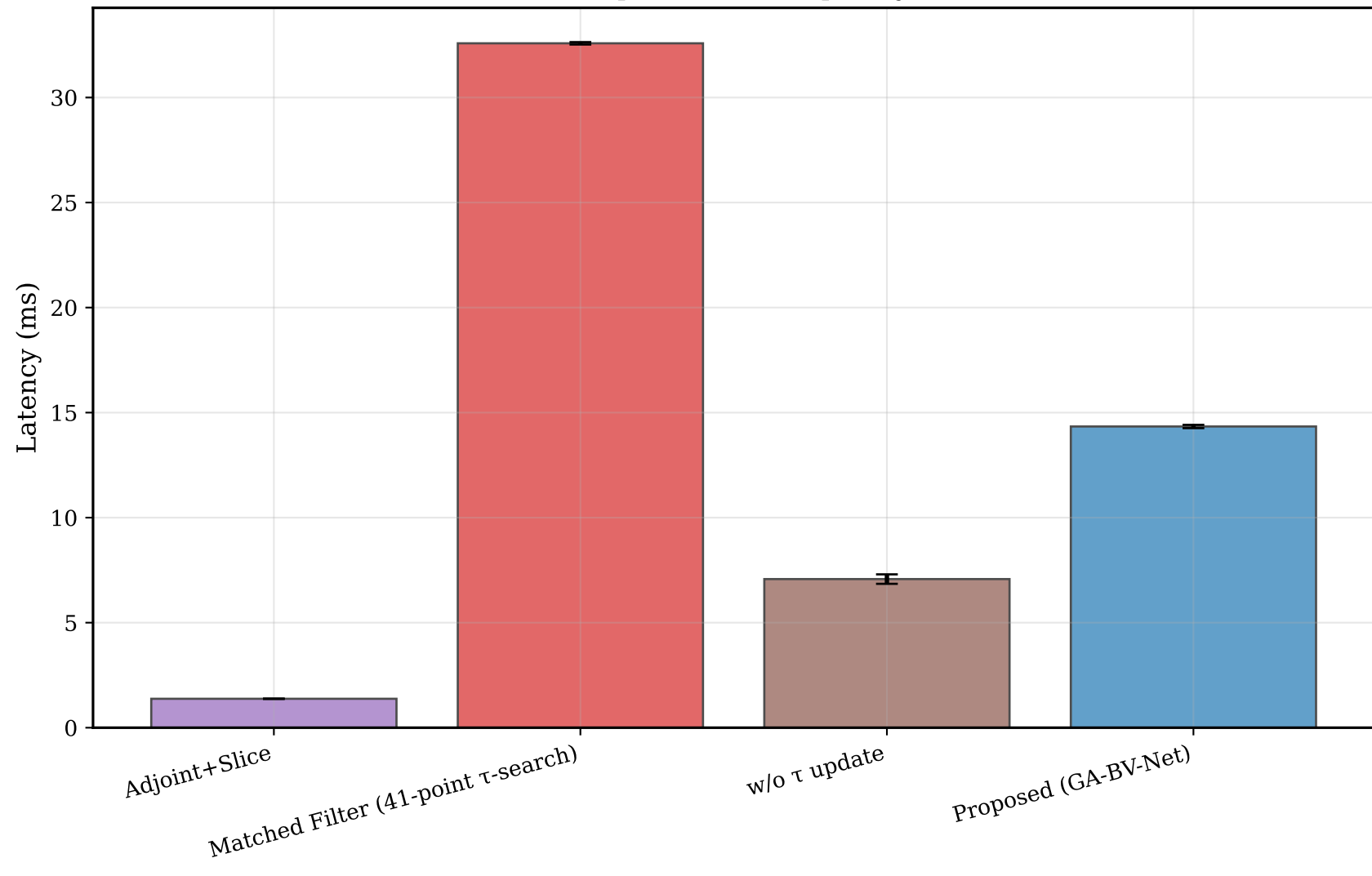
Computational Complexity
