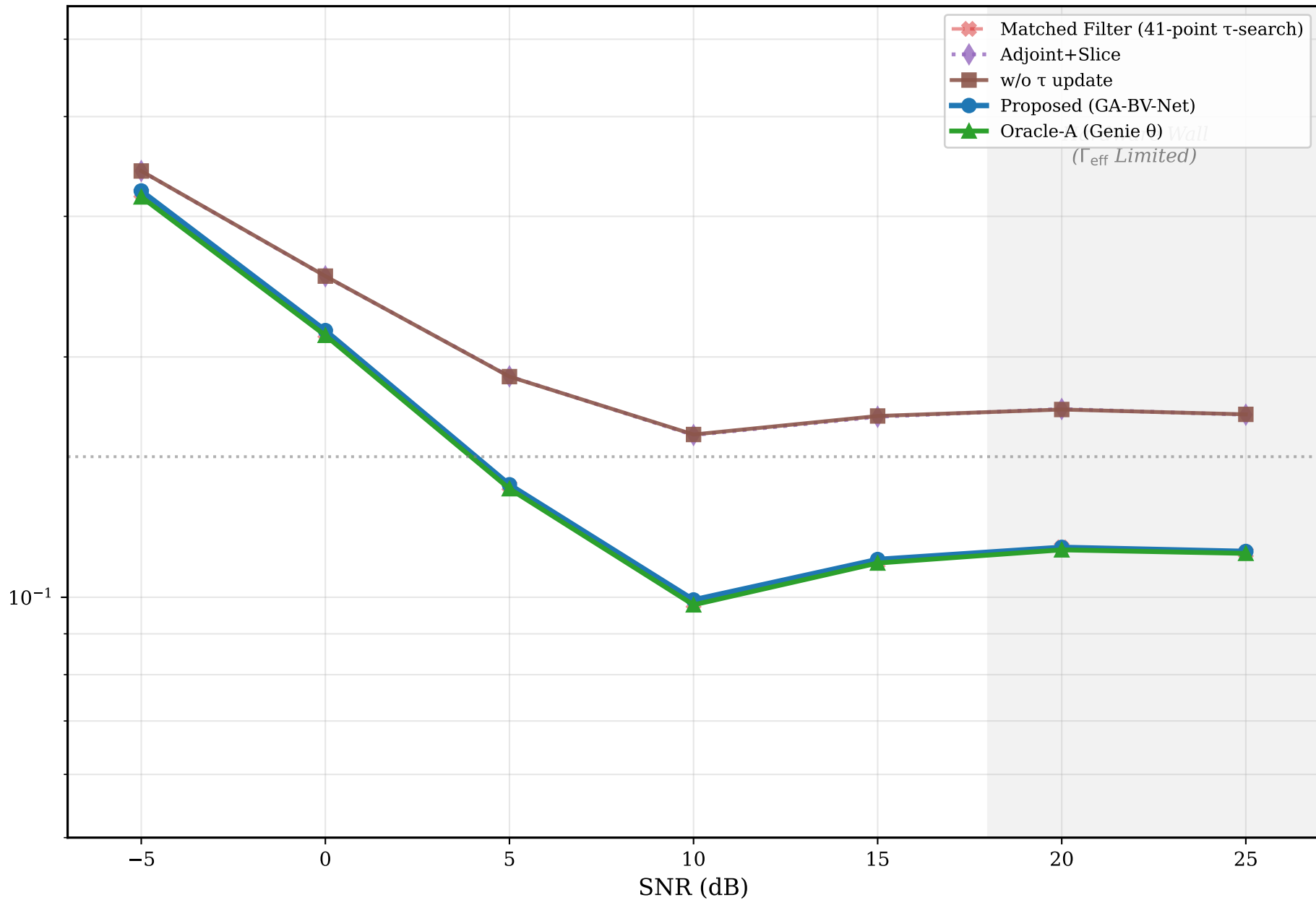
Communication Performance: BER vs SNR
