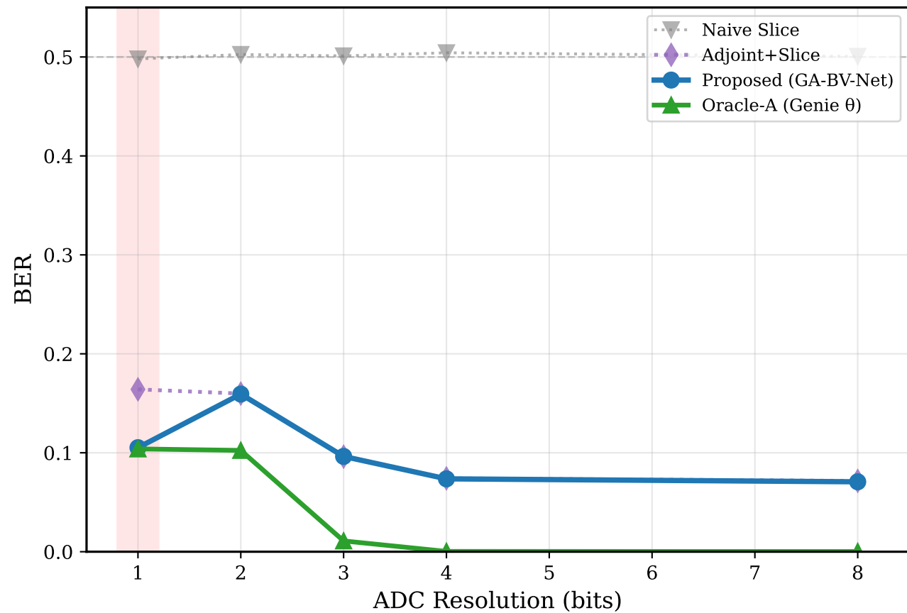
(a) BER vs ADC Bits: 1-bit Cliff
