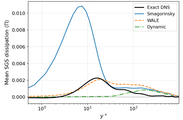
Fig. 23 Wall-normal profile of mean SGS dissipation \langle \Pi \rangle(y^+) for channel flow ( Re_\tau = 1000 ).
