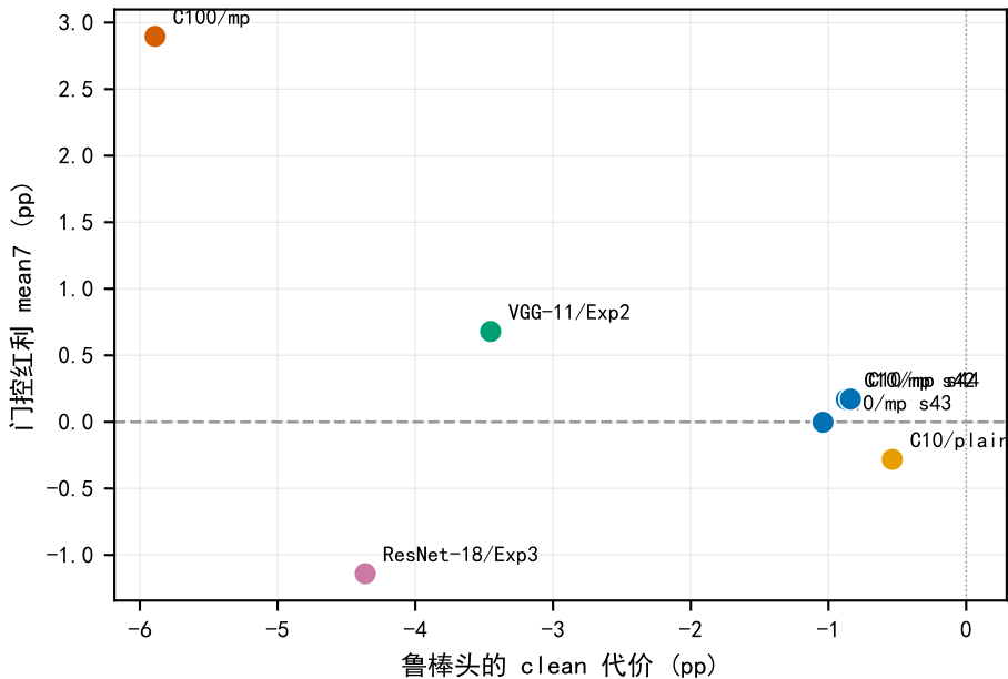
七个点，逐点 Pearson r = -0.533
