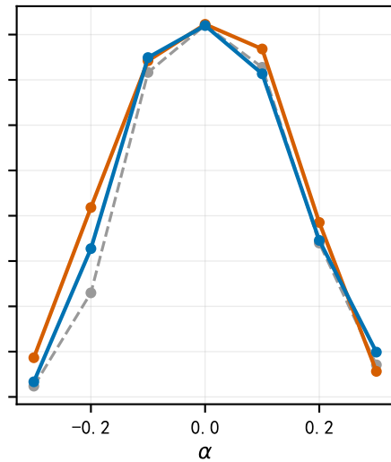
ResNet-18
