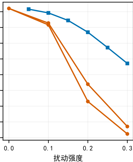
ResNet-18
