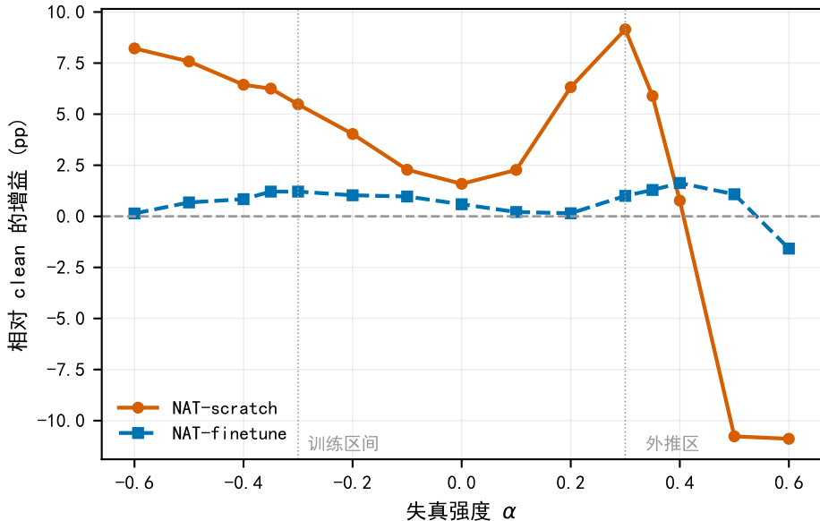
SimpleCNN / CIFAR-10 (横轴 \pm 0.6 , 15 点)
