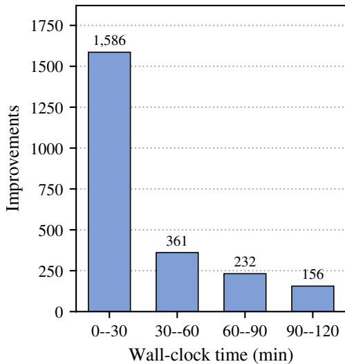
(a) Incumbent updates
