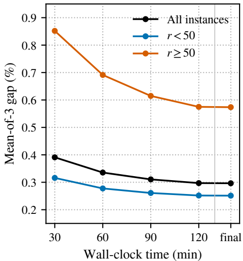
(b) Gap by route band
