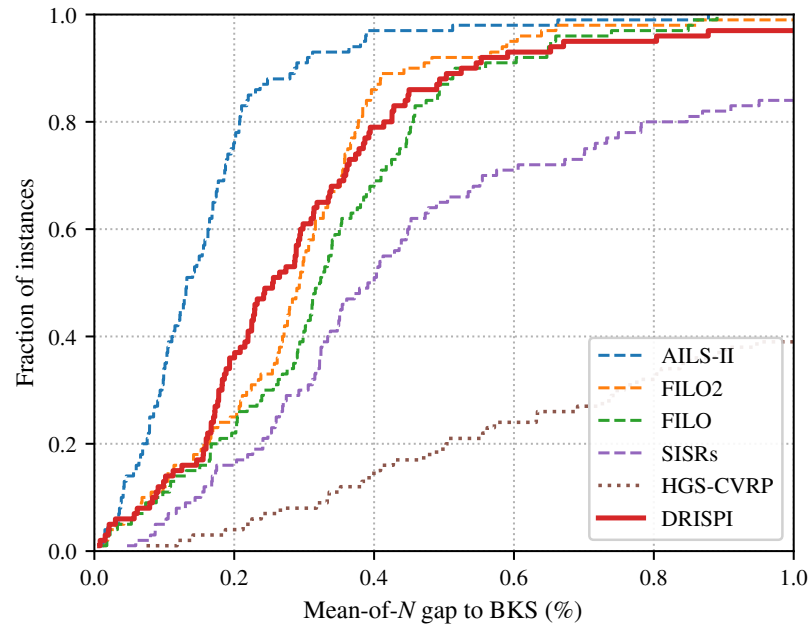
Figure 4.1: Empirical CDF of the mean-of- N gap to the current BKS. KGLSXXL, LKH-3, and OR-Tools are omitted (Section 4.2.1): their gaps would compress the visible range for the other six.
