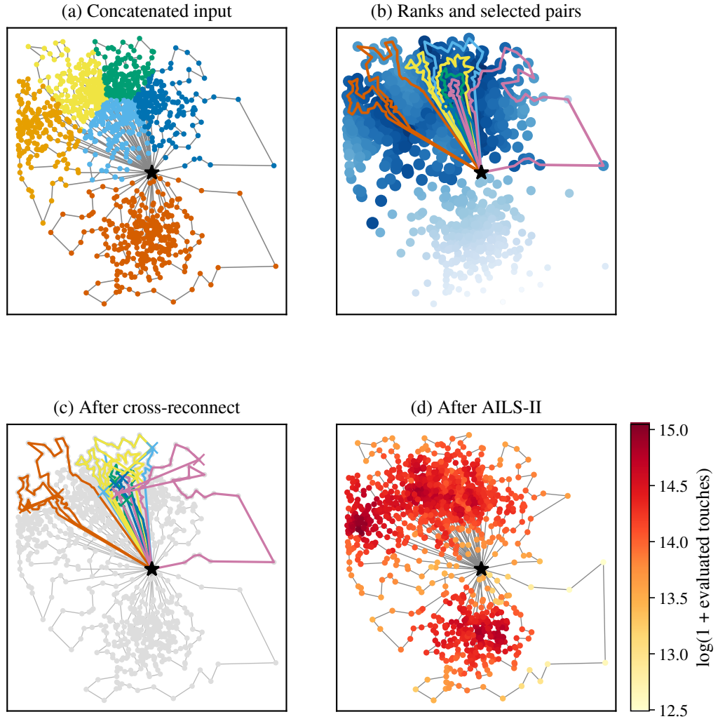
Figure 3.2: One BG-AILS call on XL-n1281-k29 (seed 101, T = 60 s). Colorbar applies to panel (d) only.
