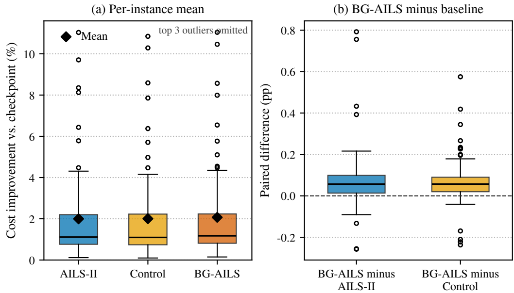
Figure 3.3: Per-instance mean cost improvement (a) and paired BG-AILS differences (b). Top three outliers omitted in (a).
