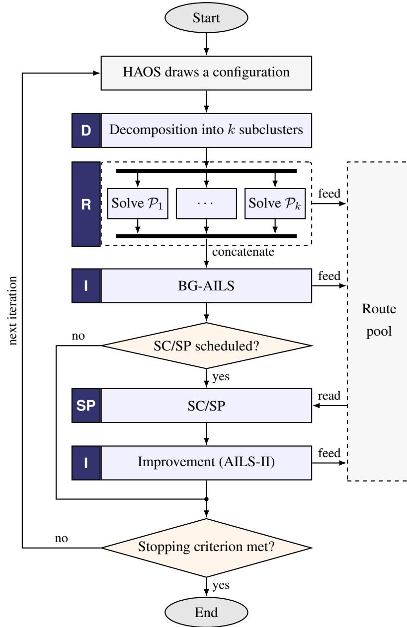
Figure 3.1: Sequential control flow of one DRISPI run: the DRI loop, the route pool, and periodic SC/SP recombination.
