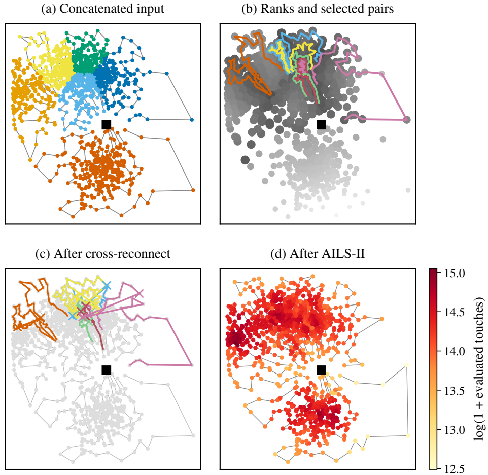
Figure 3.2: Illustrative BG-AILS Call on Instance XL-n1281-k29. Colorbar Applies to Panel (d) Only.
