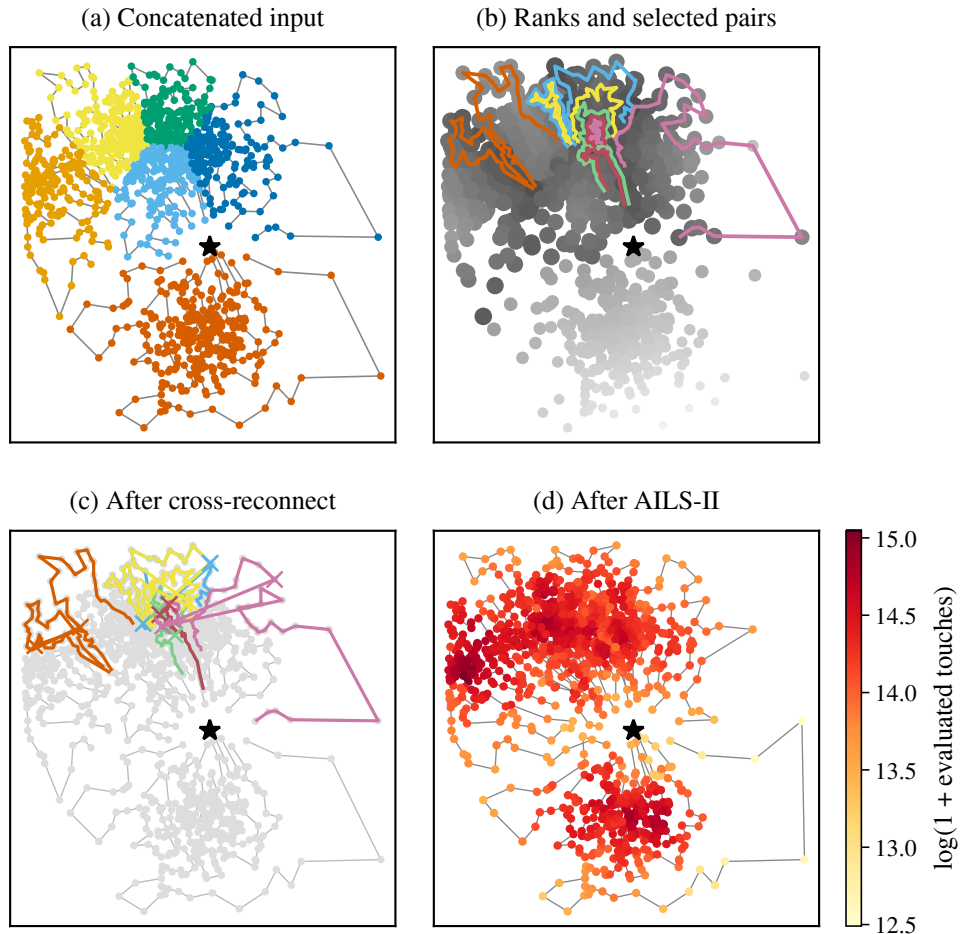
Figure 3.2: Illustrative BG-AILS Call on Instance XL-n1281-k29.
