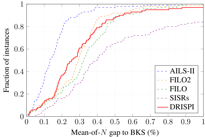
Figure 5.1: Empirical cumulative distribution of the mean-of- N gap to the current BKS, for the five solvers with a mean-of- N gap below one percent in Table 5.1.
