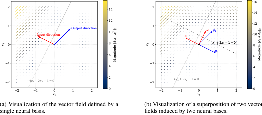
Figure 1: Geometric interpretation of neural bases from the perspective of vector fields. (a) Visualization of a single neural basis, defined by the function \phi(x) = \sigma(\langle x, s \rangle + b)p with parameters s = (-4, 2) , b = -1 , and p = (1, 1) . The red and blue arrows indicate the directions of sensor s and response p in the input and output vector fields, respectively. The dashed line marks the decision boundary induced by the equation \langle x, s \rangle + b = 0 . The small arrows on the grid illustrate the push-forward effect of the vector field. (b) A superposition of two vector fields, where the first neural basis is the same as that shown in (a) and the second basis has parameters s_2 = (1, 2) , b_2 = -1 , and p_2 = (2, -1) . Note that a single neuron can only cause one directional effect, whereas the combination of two neurons can generate multiple directional effects, as exhibited by the rotational dynamics in (b) .
