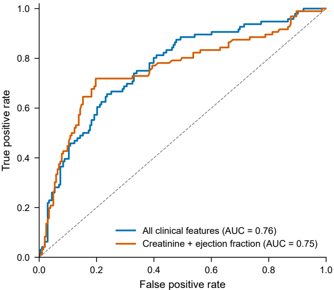
Predicting in-study death (5-fold CV)
