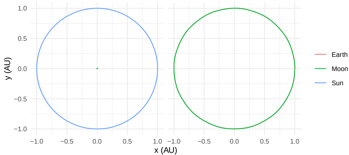
Geocentric
