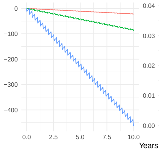
Perihelion direction (deg)
