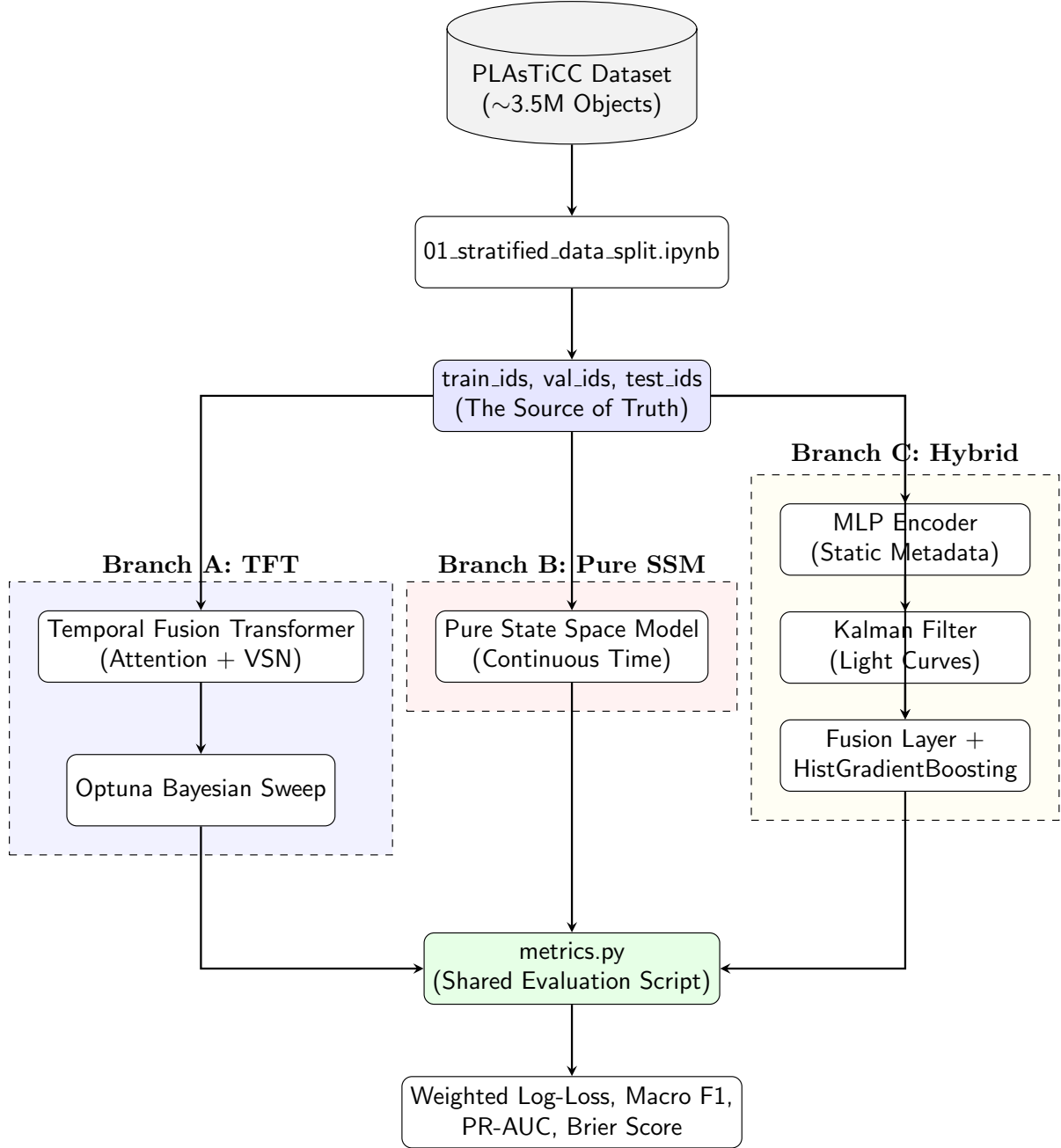
Figure 3.1: End-to-end pipeline architecture. The shared unblinded data is stratified and routed into three independent model environments before converging into a standardized evaluation script for fair benchmarking.
