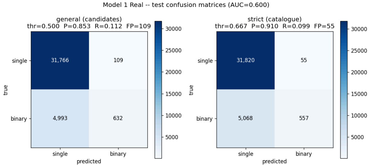
Image 15. Real version of CNN model's confusion matrices showing the general threshold on the left and the strict one on the right.
