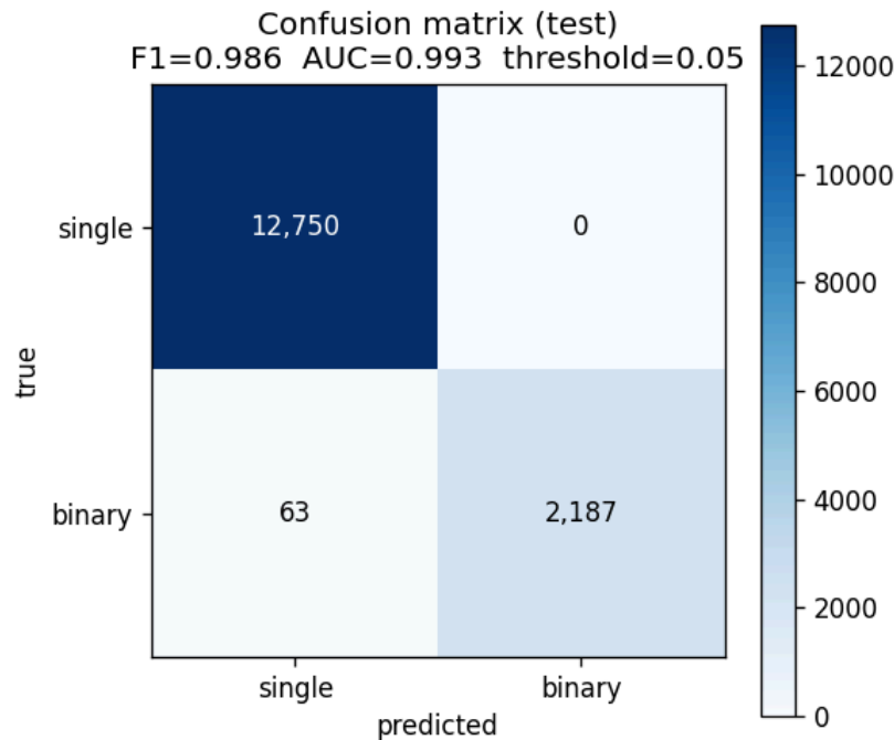
Image 14. Simple version of CNN model's confusion matrix.
