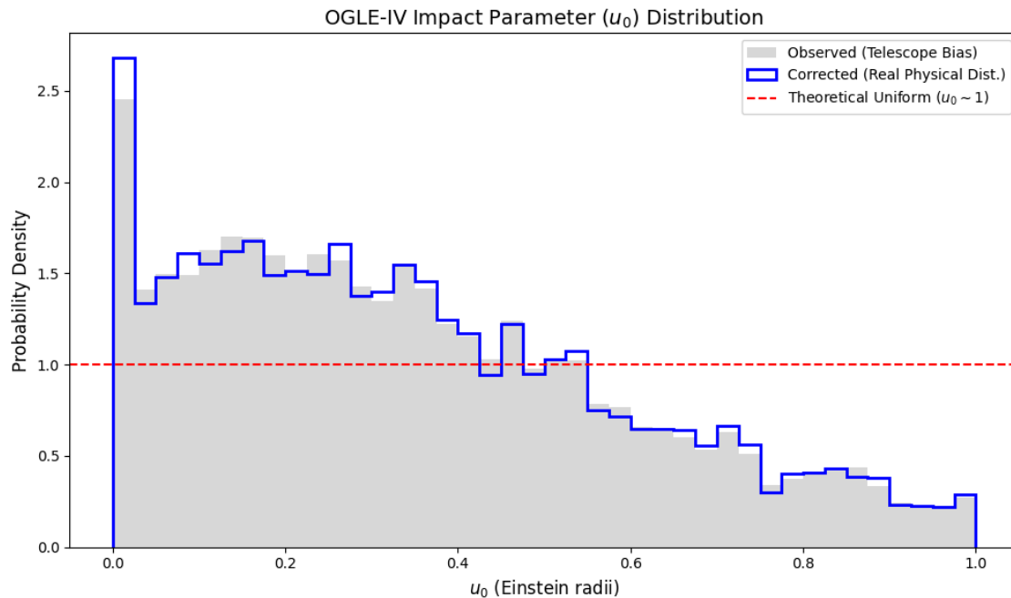
Image 7. Impact parameter distribution in a microlensing event. Source: Personal elaboration generated with python from data available at [9]
