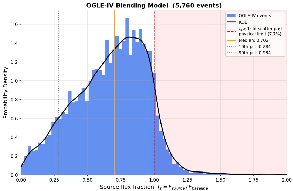
Image 13. Distribution of the OGLE-IV blend fraction f_s . Source: Personal elaboration generated with Python from data available at [30]
