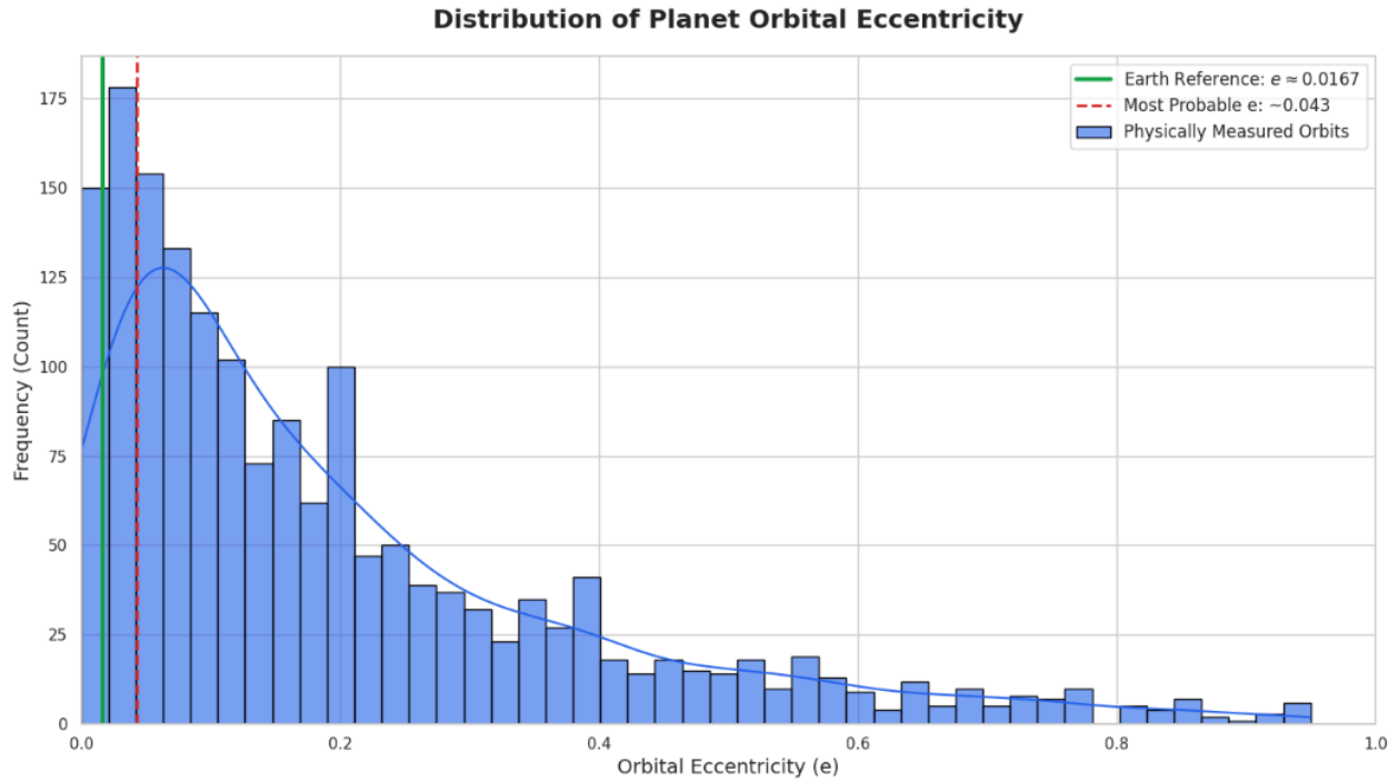
Image 9. Planet's orbital eccentricity distribution in a microlensing event. Source: Personal elaboration generated with Python from data available at [26] in column Eccentricity
