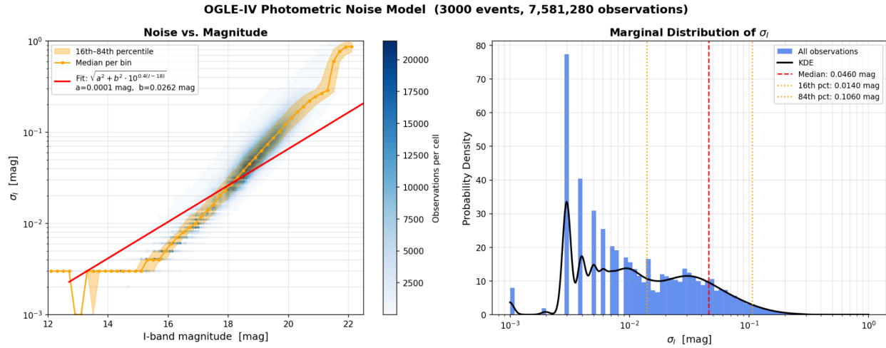
Image 11. Photometric noise model from OGLE-IV survey. Source: Personal elaboration generated with Python from data available at [29]
