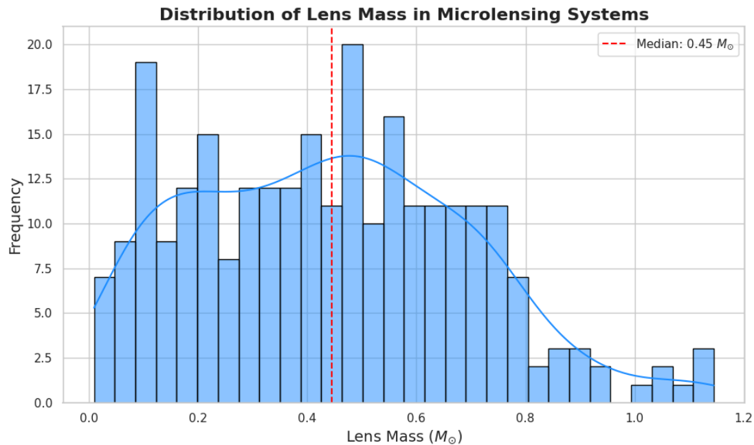
Image 2. Lens' Mass distribution in a microlensing event. Source: Personal elaboration generated with Python from data available at [25] in column Lens Mass [Solar mass]
