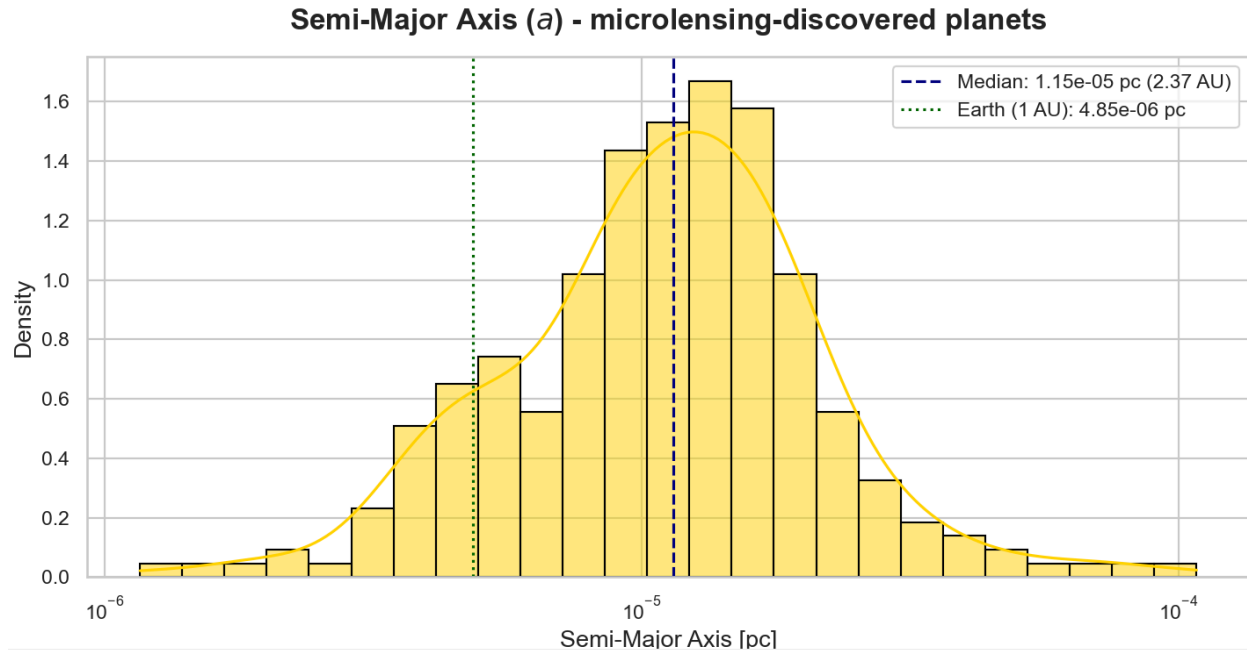
Image 8. Planet's semi-major axis distribution in a microlensing event. Source: Personal elaboration generated with Python from data available at [26] in column Orbit Semi-Major Axis [au]
