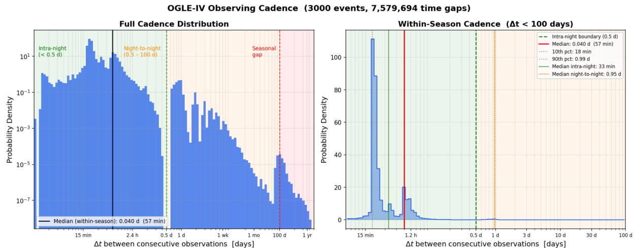
Image 12. Observing cadence model from OGLE-IV survey. Source: Personal elaboration generated with Python from data available at [29]
