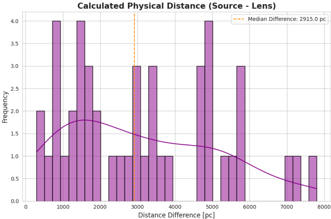
Image 4. Lens to Source Distance distribution in a microlensing event. Source: Personal elaboration generated with Python from data available at [25] in columns Lens Distance [pc] and Source Distance [pc]
