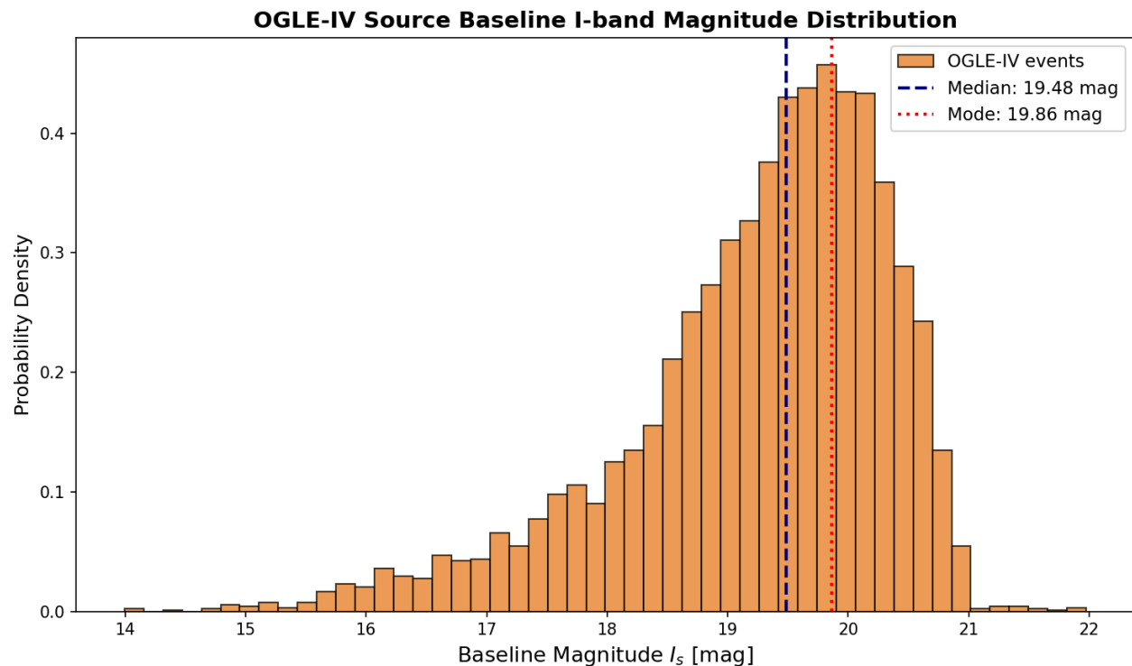
Image 10. OGLE-IV survey extracted source baseline I-band magnitude distribution. Source: Personal elaboration generated with Python from data available at [30]
