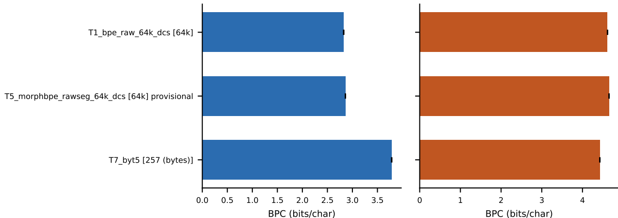
track1 · smoke · in-domain (DCS held out)
