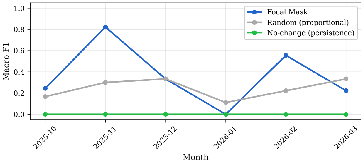
Macro F1 by month — Transition cells only
