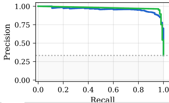
Macro PR
