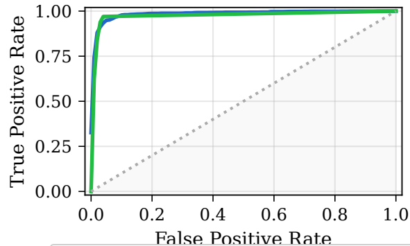
Macro ROC
