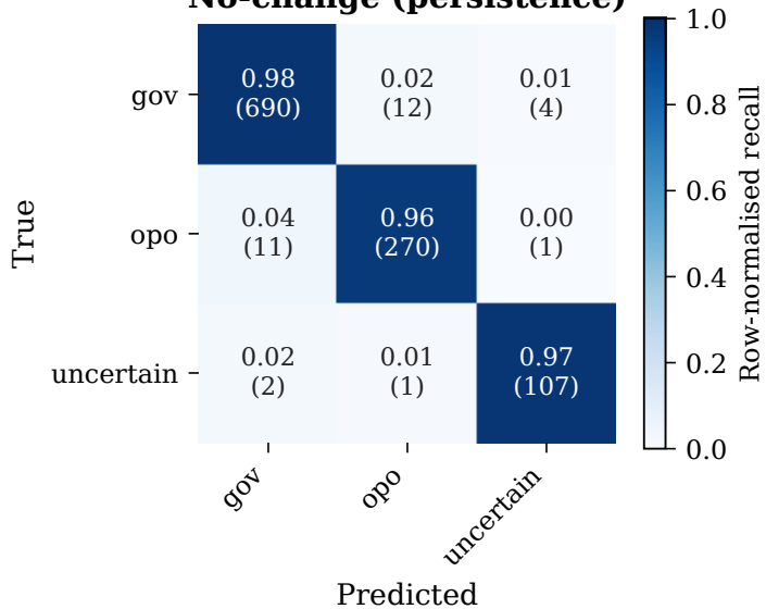
No-change (persistence)
